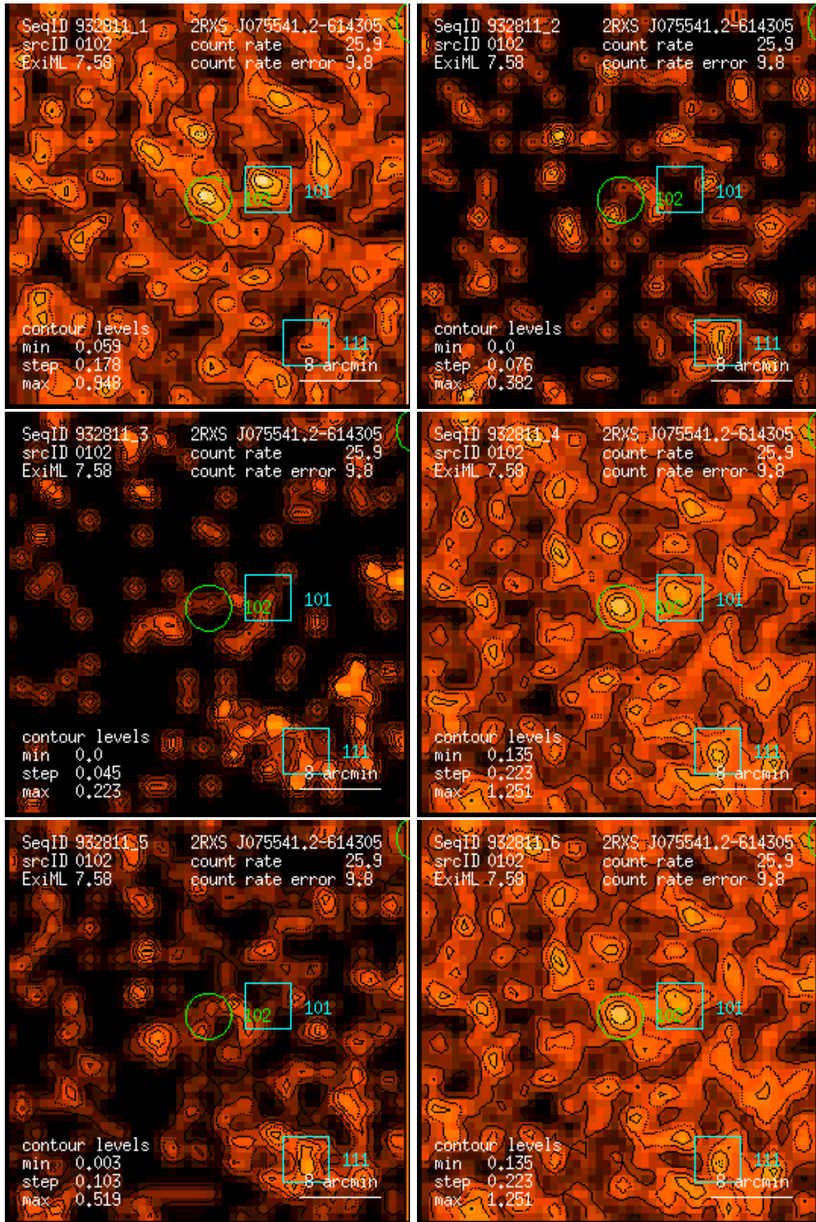
Figure 102: RASS 932811: detection 0102: band rate images, Gaussian filter: (1) PSPC channels 11 – 41, (2) 52 – 90, (3) 91 – 201, (4) 11 – 235, (5) 52 – 201, (6) 11 – 201. Broad band rates in counts/ks. Band rate contour levels in counts/ks/arcmin 2 .
