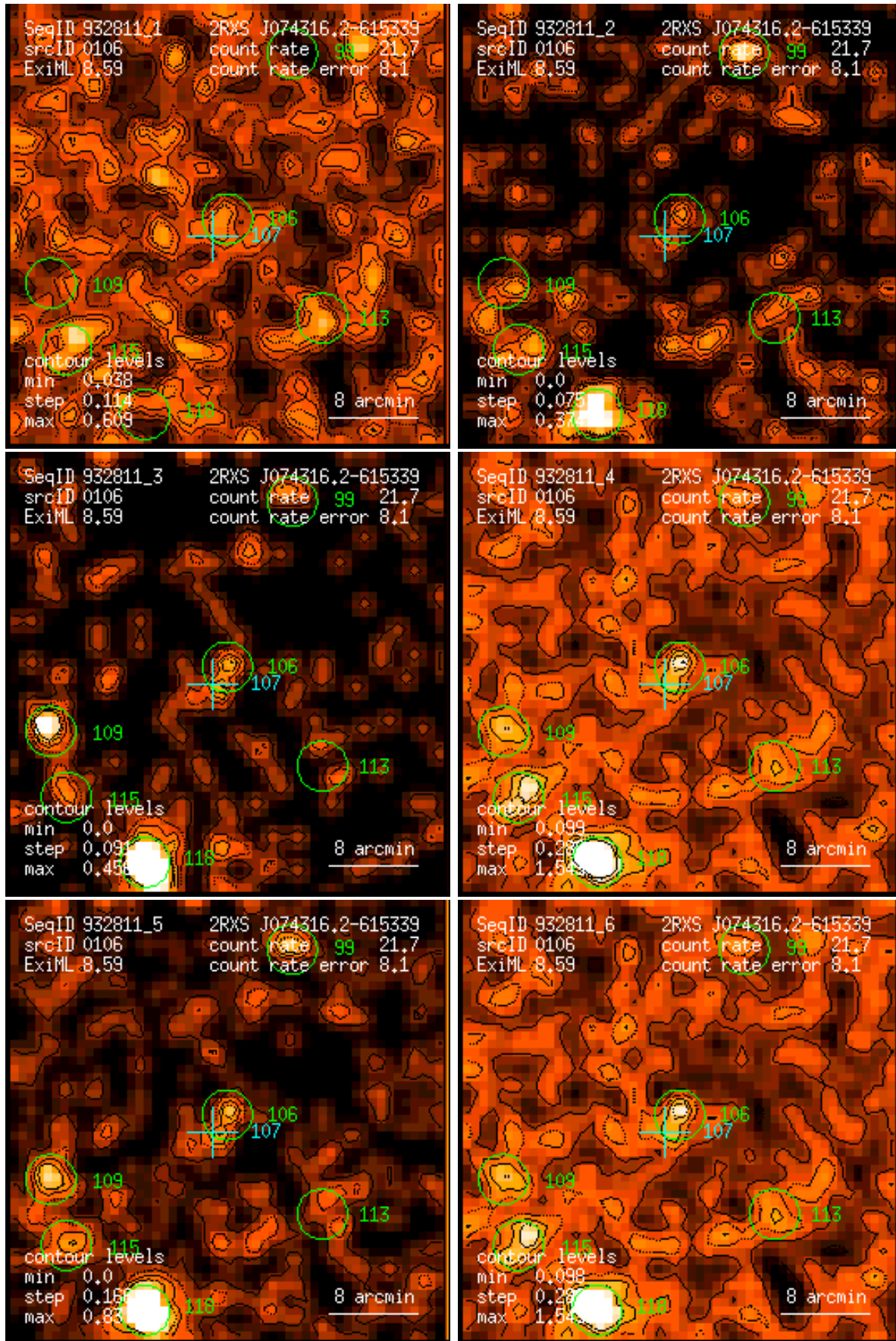
Figure 106: RASS 932811: detection 0106: band rate images, Gaussian filter: (1) PSPC channels 11 – 41, (2) 52 – 90, (3) 91 – 201, (4) 11 – 235, (5) 52 – 201, (6) 11 – 201. Broad band rates in counts/ks. Band rate contour levels in counts/ks/arcmin 2 .
