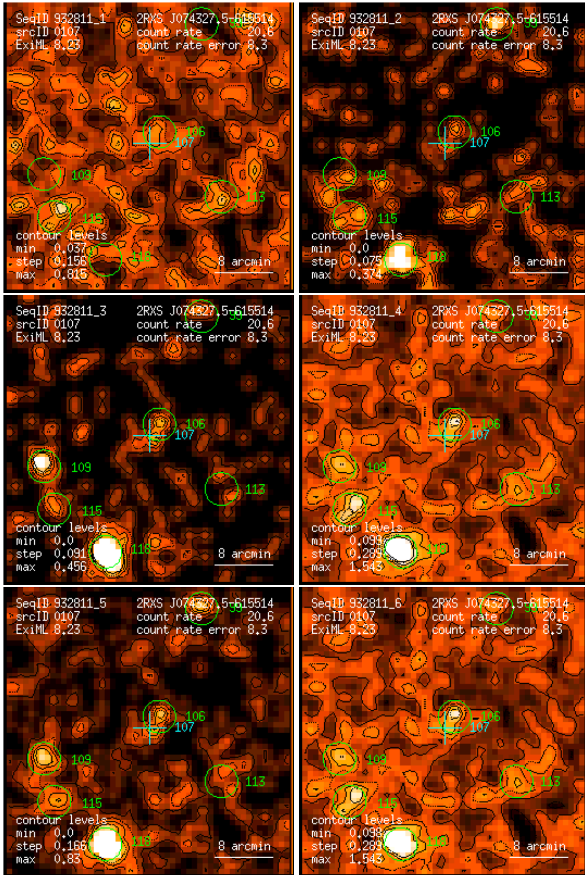
Figure 107: RASS 932811: detection 0107: band rate images, Gaussian filter: (1) PSPC channels 11 – 41, (2) 52 – 90, (3) 91 – 201, (4) 11 – 235, (5) 52 – 201, (6) 11 – 201. Broad band rates in counts/ks. Band rate contour levels in counts/ks/arcmin 2 .
