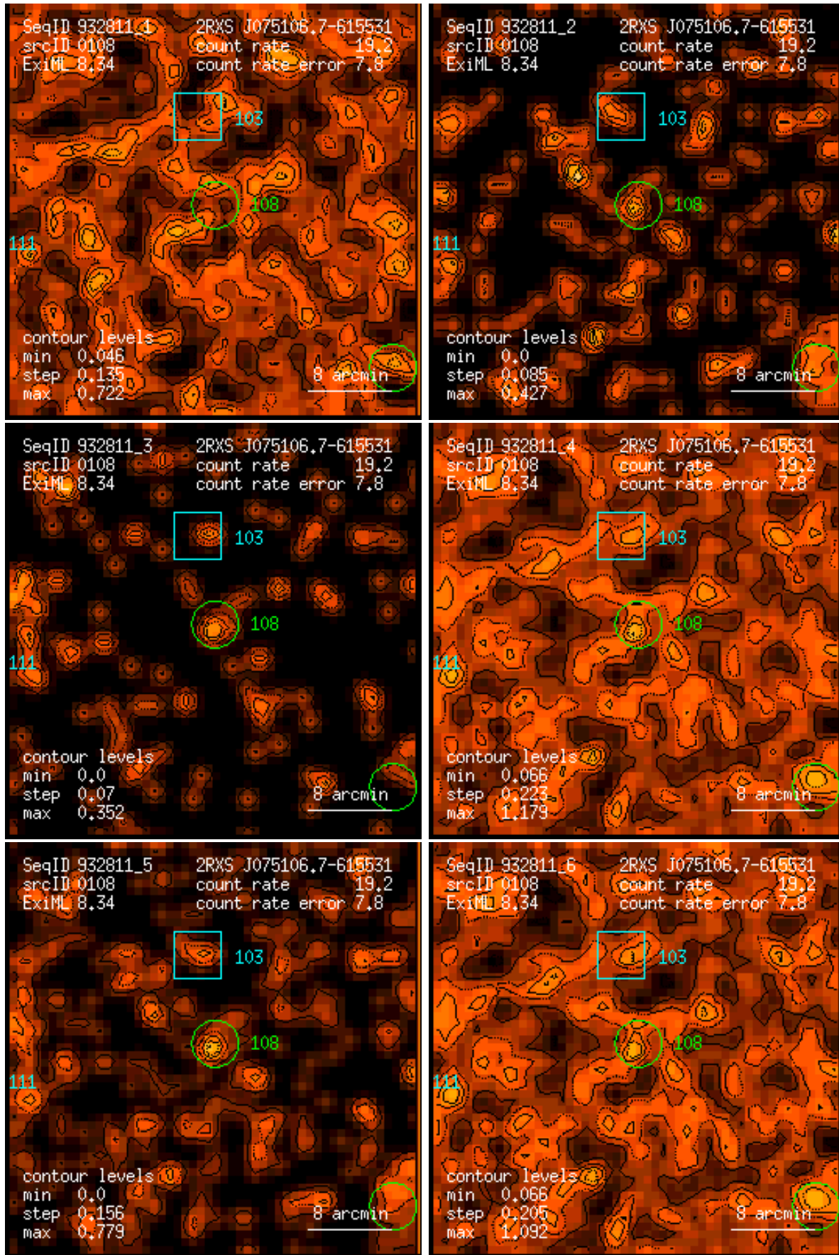
Figure 108: RASS 932811: detection 0108: band rate images, Gaussian filter: (1) PSPC channels 11 – 41, (2) 52 – 90, (3) 91 – 201, (4) 11 – 235, (5) 52 – 201, (6) 11 – 201. Broad band rates in counts/ks. Band rate contour levels in counts/ks/arcmin 2 .
