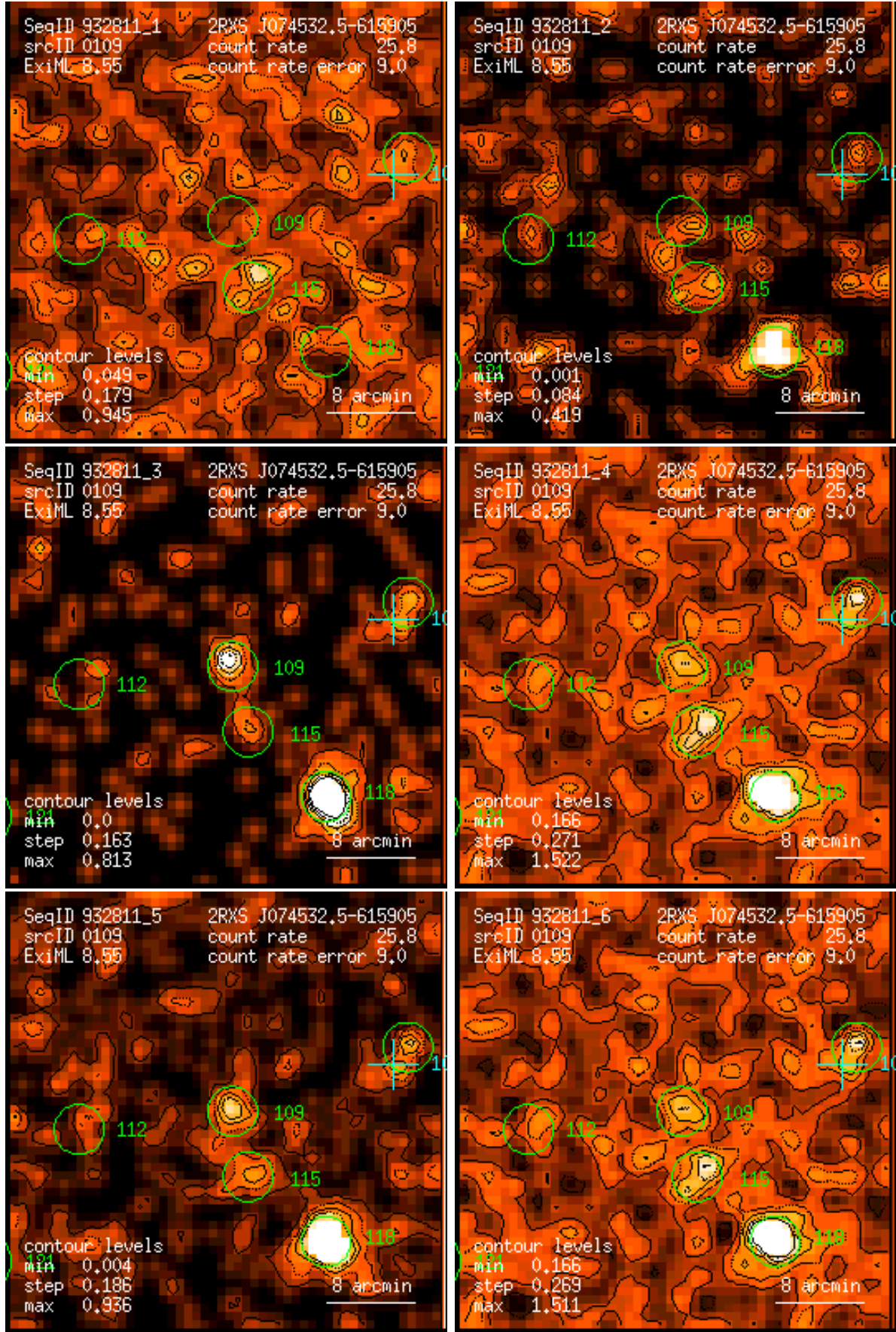
Figure 109: RASS 932811: detection 0109: band rate images, Gaussian filter: (1) PSPC channels 11 – 41, (2) 52 – 90, (3) 91 – 201, (4) 11 – 235, (5) 52 – 201, (6) 11 – 201. Broad band rates in counts/ks. Band rate contour levels in counts/ks/arcmin 2 .
