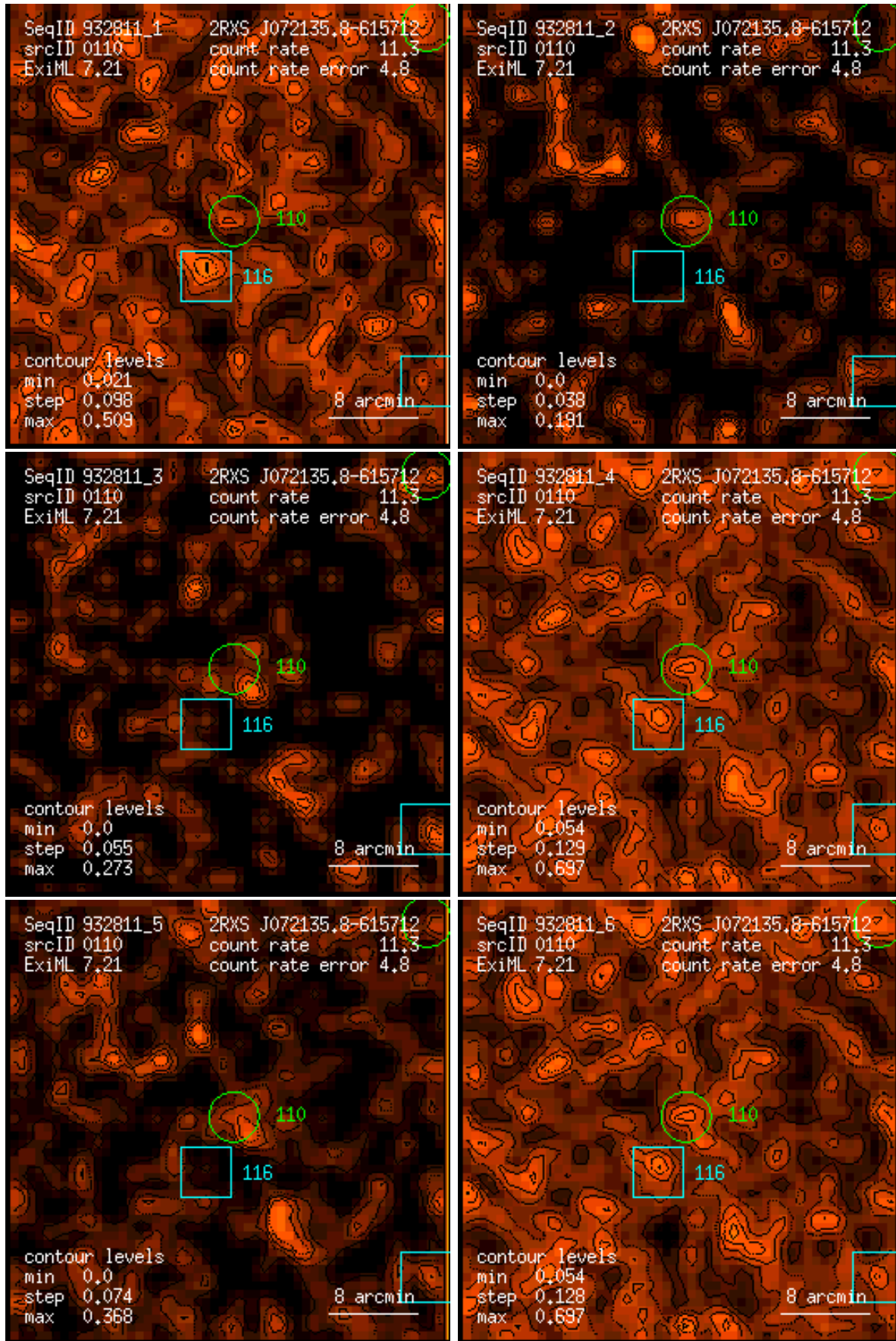
Figure 110: RASS 932811: detection 0110: band rate images, Gaussian filter: (1) PSPC channels 11 – 41, (2) 52 – 90, (3) 91 – 201, (4) 11 – 235, (5) 52 – 201, (6) 11 – 201. Broad band rates in counts/ks. Band rate contour levels in counts/ks/arcmin 2 .
