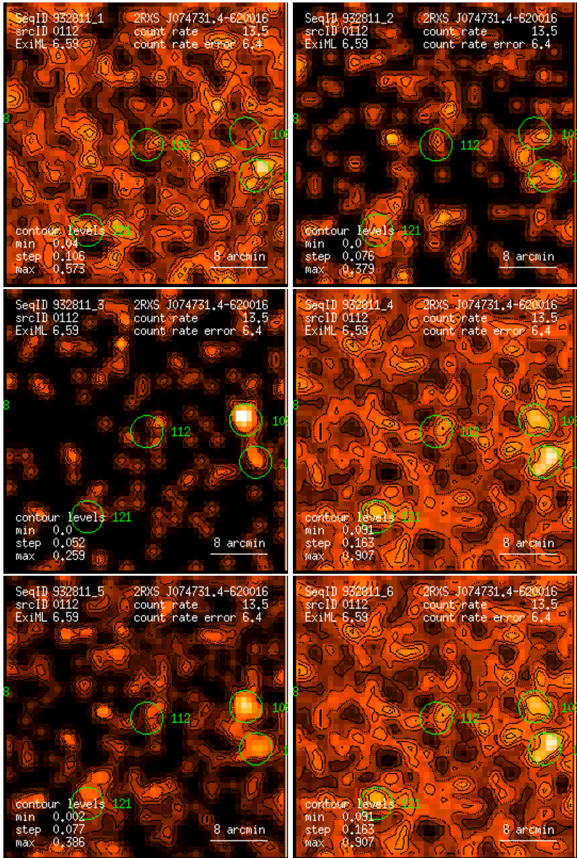
Figure 112: RASS 932811: detection 0112: band rate images, Gaussian filter: (1) PSPC channels 11 – 41, (2) 52 – 90, (3) 91 – 201, (4) 11 – 235, (5) 52 – 201, (6) 11 – 201. Broad band rates in counts/ks. Band rate contour levels in counts/ks/arcmin 2 .
