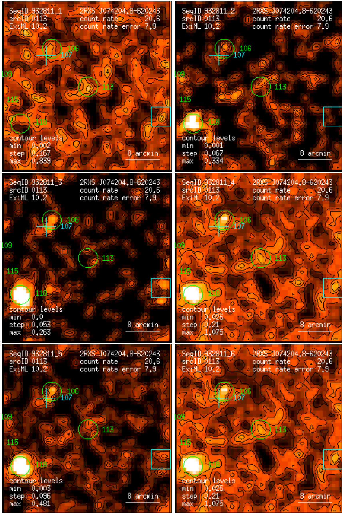
Figure 113: RASS 932811: detection 0113: band rate images, Gaussian filter: (1) PSPC channels 11 – 41, (2) 52 – 90, (3) 91 – 201, (4) 11 – 235, (5) 52 – 201, (6) 11 – 201. Broad band rates in counts/ks. Band rate contour levels in counts/ks/arcmin 2 .
