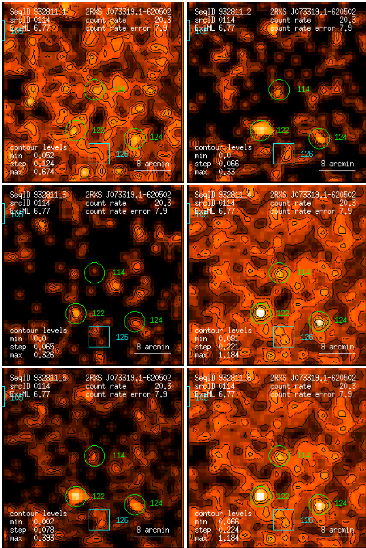
Figure 114: RASS 932811: detection 0114: band rate images, Gaussian filter: (1) PSPC channels 11 – 41, (2) 52 – 90, (3) 91 – 201, (4) 11 – 235, (5) 52 – 201, (6) 11 – 201. Broad band rates in counts/ks. Band rate contour levels in counts/ks/arcmin 2 .
