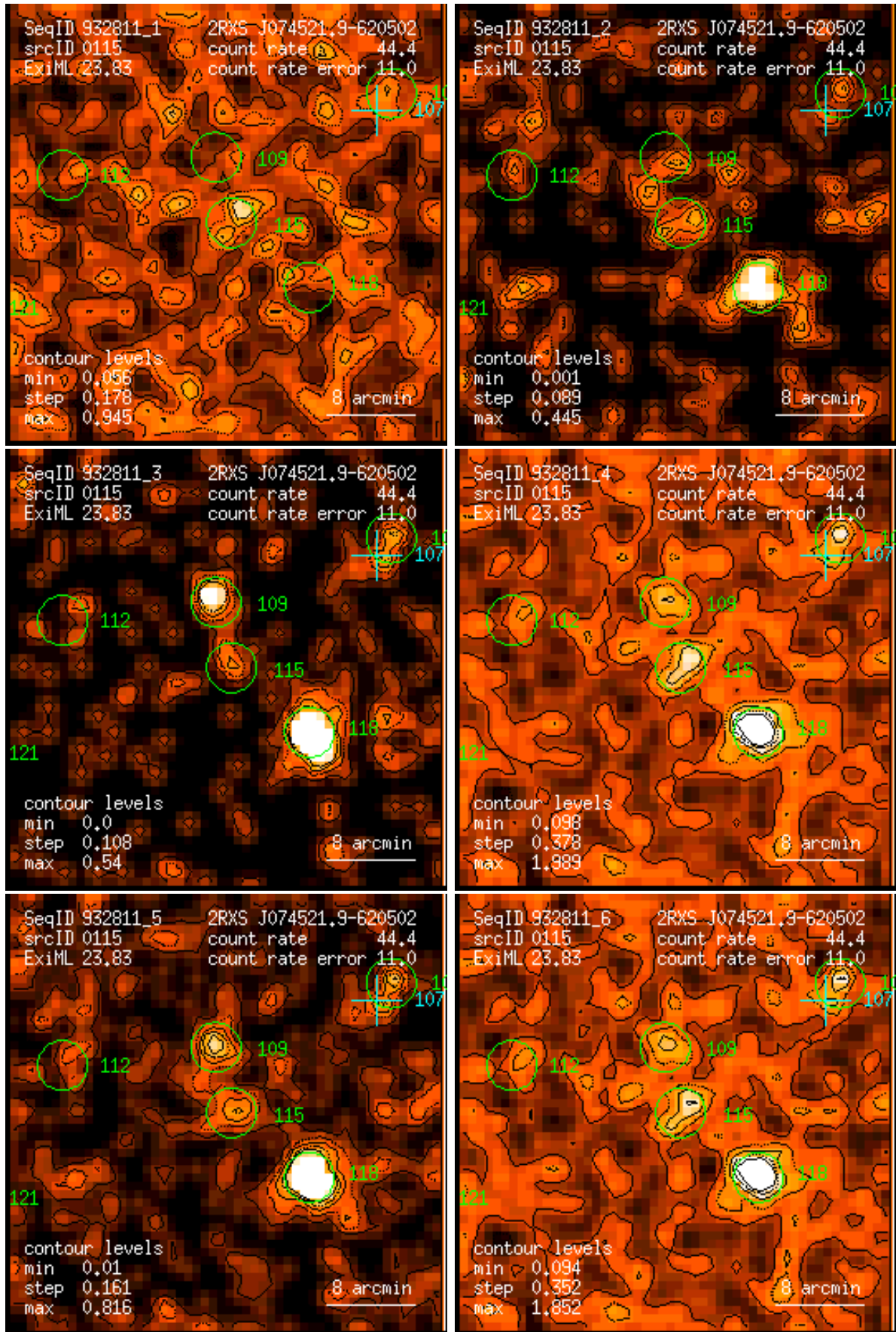
Figure 115: RASS 932811: detection 0115: band rate images, Gaussian filter: (1) PSPC channels 11 – 41, (2) 52 – 90, (3) 91 – 201, (4) 11 – 235, (5) 52 – 201, (6) 11 – 201. Broad band rates in counts/ks. Band rate contour levels in counts/ks/arcmin 2 .
