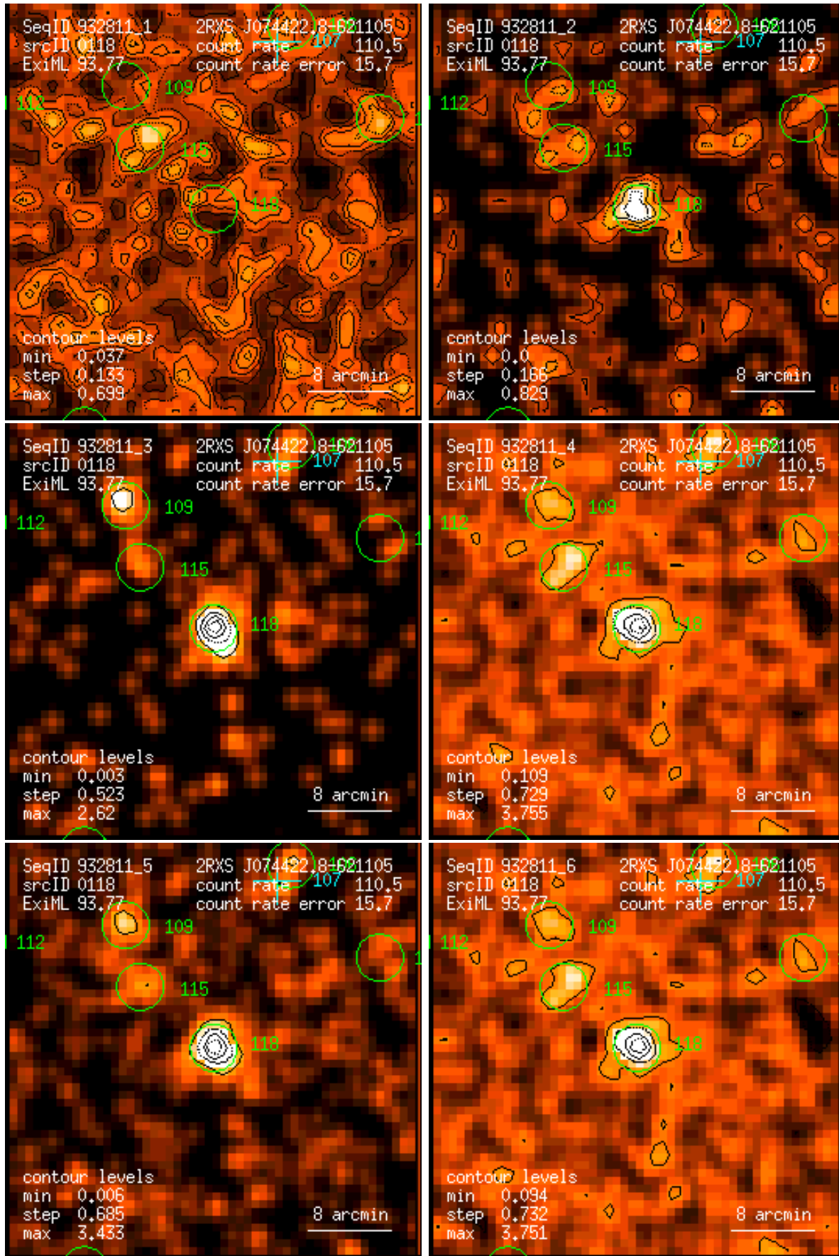
Figure 118: RASS 932811: detection 0118: band rate images, Gaussian filter: (1) PSPC channels 11 – 41, (2) 52 – 90, (3) 91 – 201, (4) 11 – 235, (5) 52 – 201, (6) 11 – 201. Broad band rates in counts/ks. Band rate contour levels in counts/ks/arcmin 2 .
