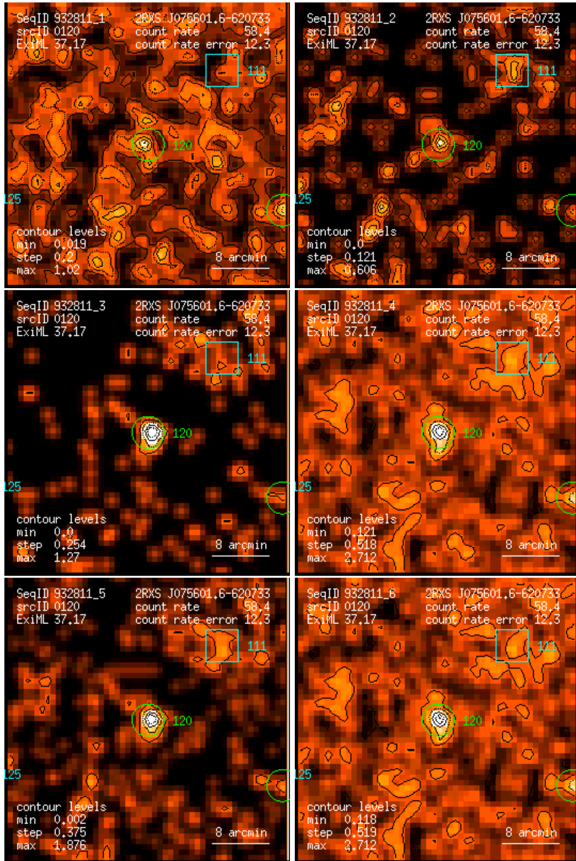
Figure 120: RASS 932811: detection 0120: band rate images, Gaussian filter: (1) PSPC channels 11 – 41, (2) 52 – 90, (3) 91 – 201, (4) 11 – 235, (5) 52 – 201, (6) 11 – 201. Broad band rates in counts/ks. Band rate contour levels in counts/ks/arcmin 2 .
