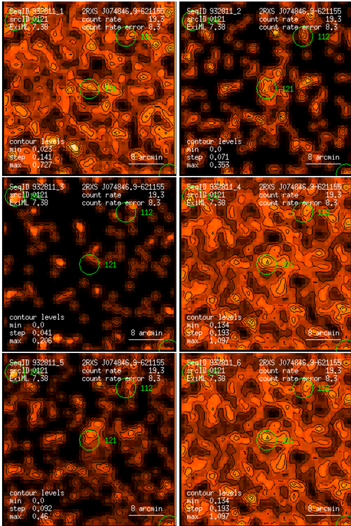
Figure 121: RASS 932811: detection 0121: band rate images, Gaussian filter: (1) PSPC channels 11 – 41, (2) 52 – 90, (3) 91 – 201, (4) 11 – 235, (5) 52 – 201, (6) 11 – 201. Broad band rates in counts/ks. Band rate contour levels in counts/ks/arcmin 2 .
