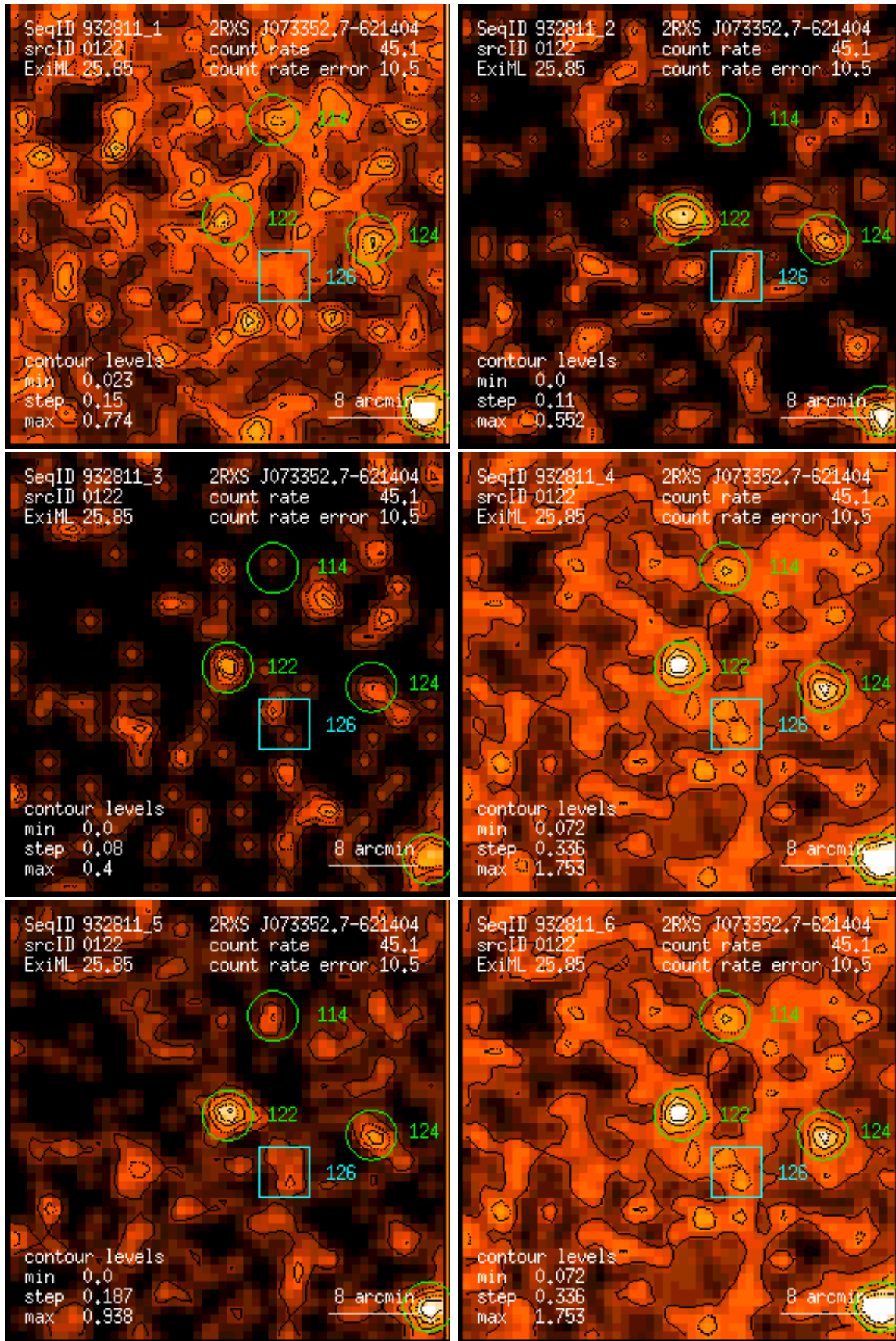
Figure 122: RASS 932811: detection 0122: band rate images, Gaussian filter: (1) PSPC channels 11 – 41, (2) 52 – 90, (3) 91 – 201, (4) 11 – 235, (5) 52 – 201, (6) 11 – 201. Broad band rates in counts/ks. Band rate contour levels in counts/ks/arcmin 2 .
