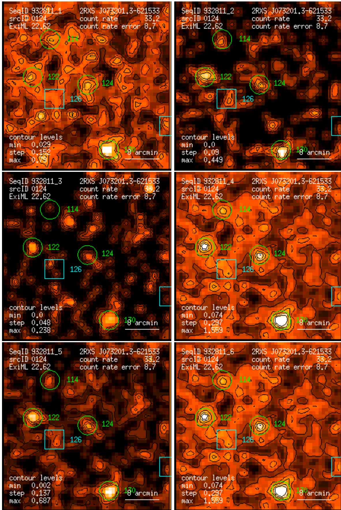
Figure 124: RASS 932811: detection 0124: band rate images, Gaussian filter: (1) PSPC channels 11 – 41, (2) 52 – 90, (3) 91 – 201, (4) 11 – 235, (5) 52 – 201, (6) 11 – 201. Broad band rates in counts/ks. Band rate contour levels in counts/ks/arcmin 2 .
