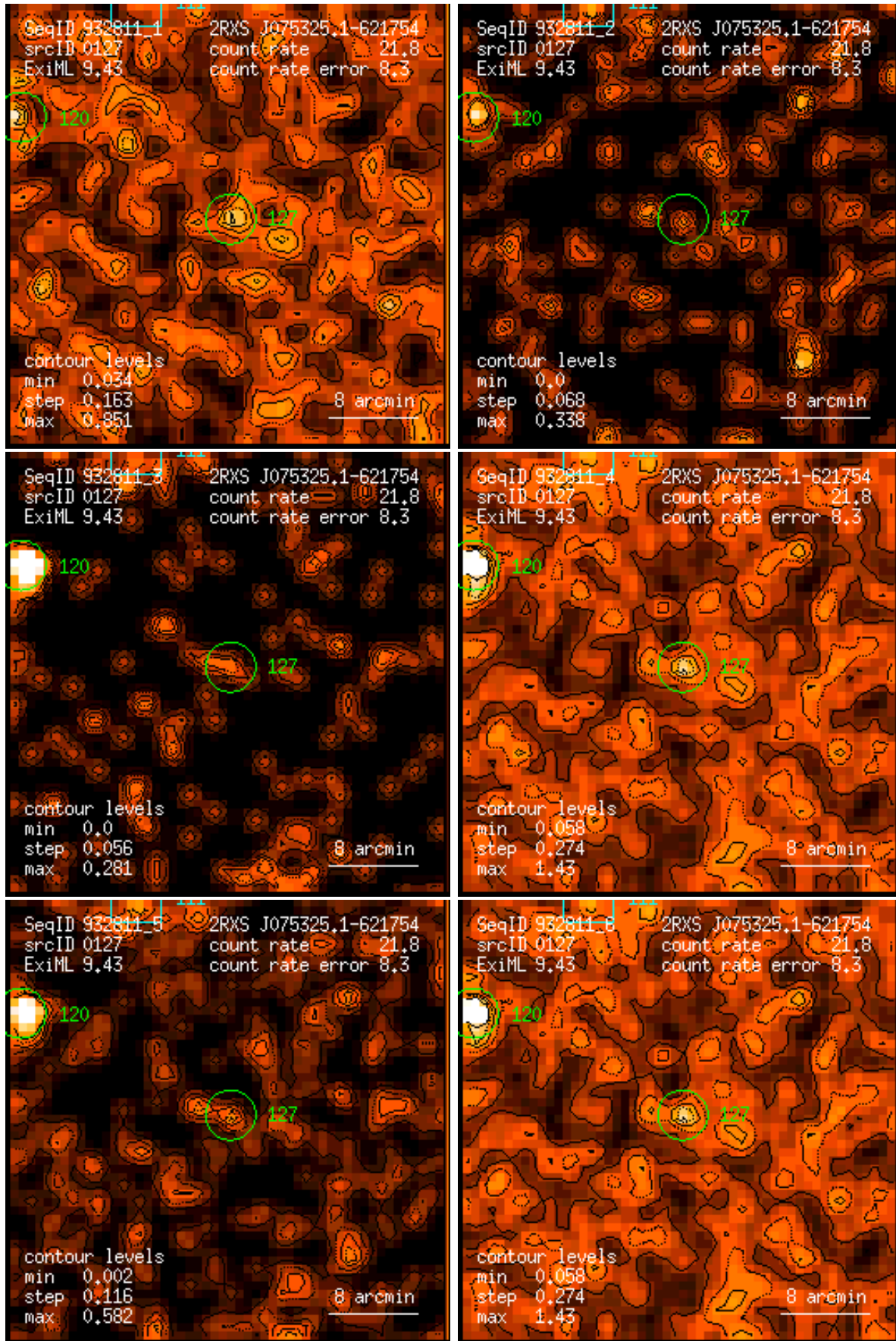
Figure 127: RASS 932811: detection 0127: band rate images, Gaussian filter: (1) PSPC channels 11 – 41, (2) 52 – 90, (3) 91 – 201, (4) 11 – 235, (5) 52 – 201, (6) 11 – 201. Broad band rates in counts/ks. Band rate contour levels in counts/ks/arcmin 2 .
