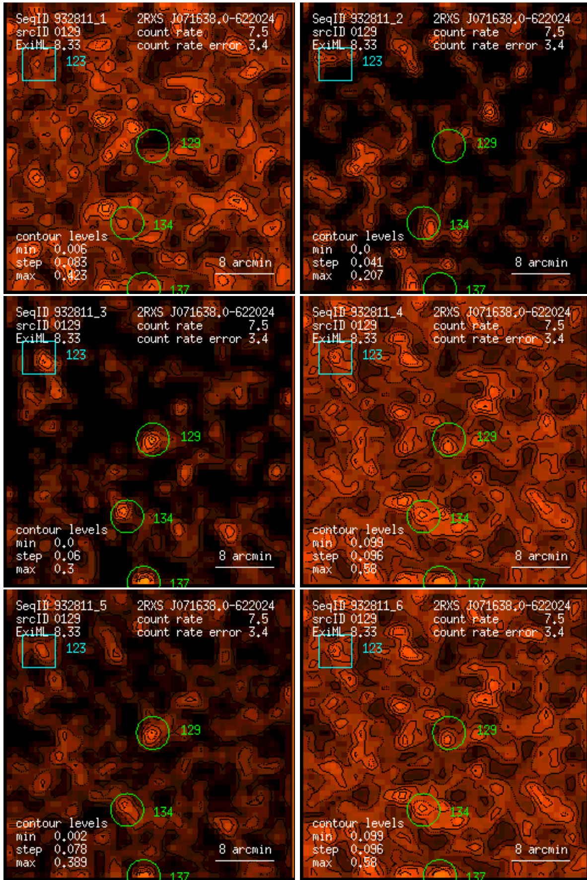
Figure 129: RASS 932811: detection 0129: band rate images, Gaussian filter: (1) PSPC channels 11 – 41, (2) 52 – 90, (3) 91 – 201, (4) 11 – 235, (5) 52 – 201, (6) 11 – 201. Broad band rates in counts/ks. Band rate contour levels in counts/ks/arcmin 2 .
