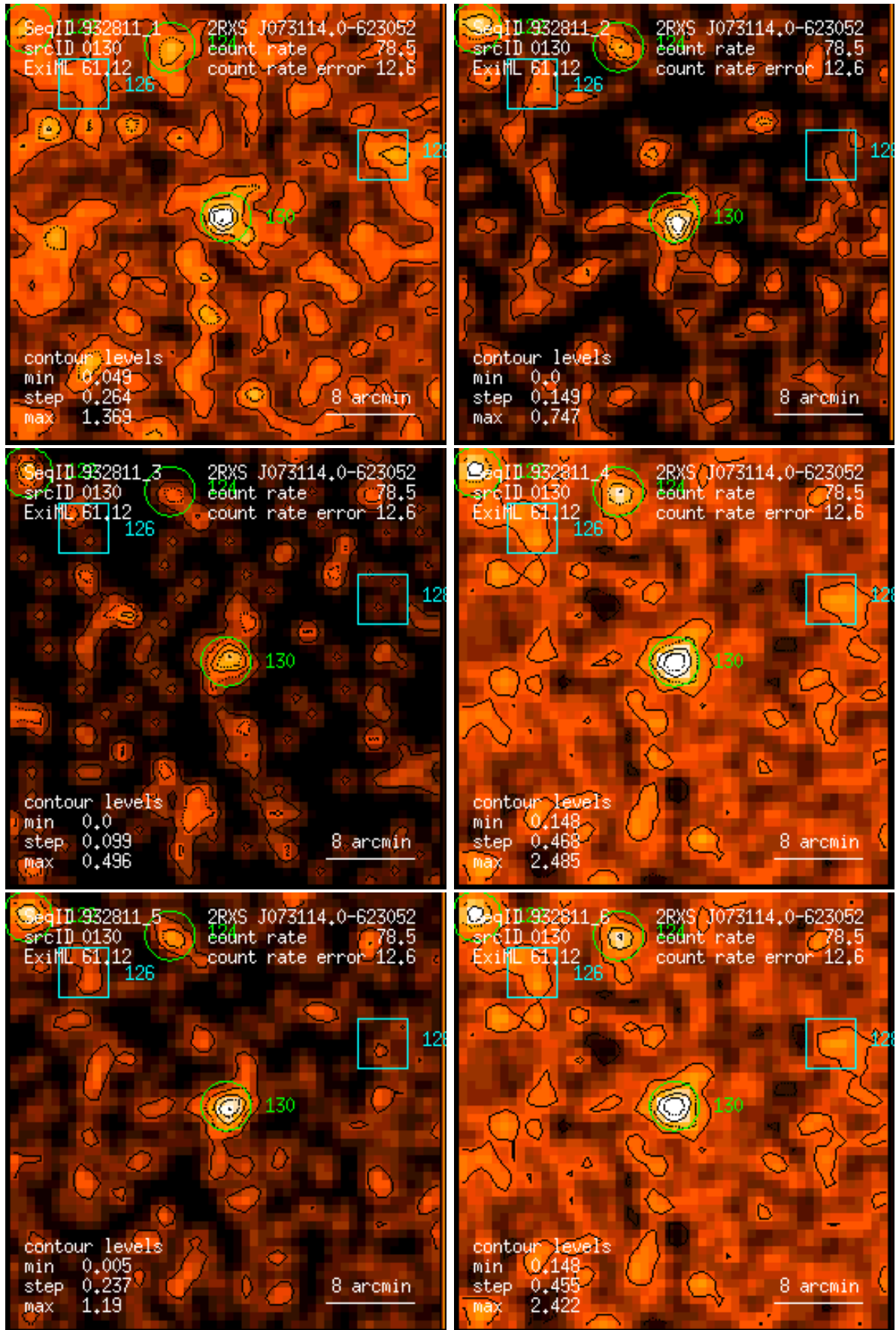
Figure 130: RASS 932811: detection 0130: band rate images, Gaussian filter: (1) PSPC channels 11 – 41, (2) 52 – 90, (3) 91 – 201, (4) 11 – 235, (5) 52 – 201, (6) 11 – 201. Broad band rates in counts/ks. Band rate contour levels in counts/ks/arcmin 2 .
