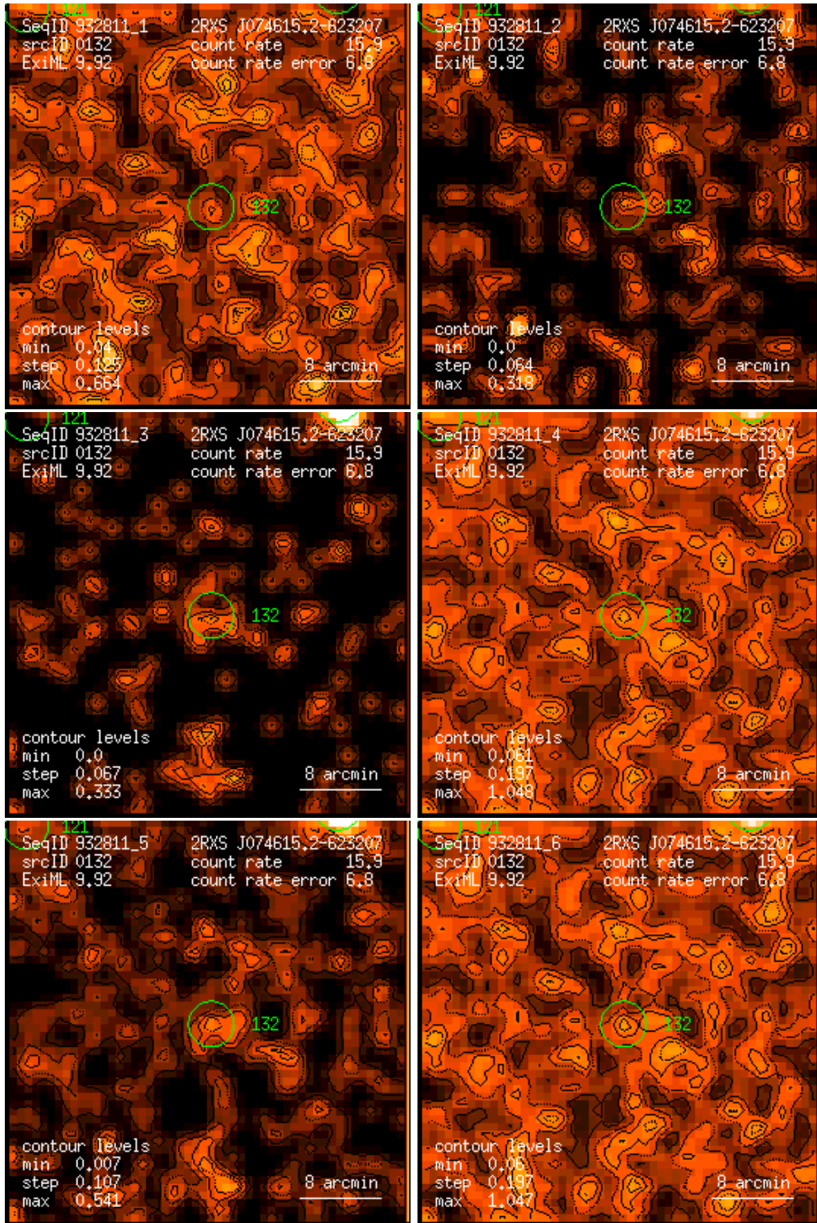
Figure 132: RASS 932811: detection 0132: band rate images, Gaussian filter: (1) PSPC channels 11 – 41, (2) 52 – 90, (3) 91 – 201, (4) 11 – 235, (5) 52 – 201, (6) 11 – 201. Broad band rates in counts/ks. Band rate contour levels in counts/ks/arcmin 2 .
