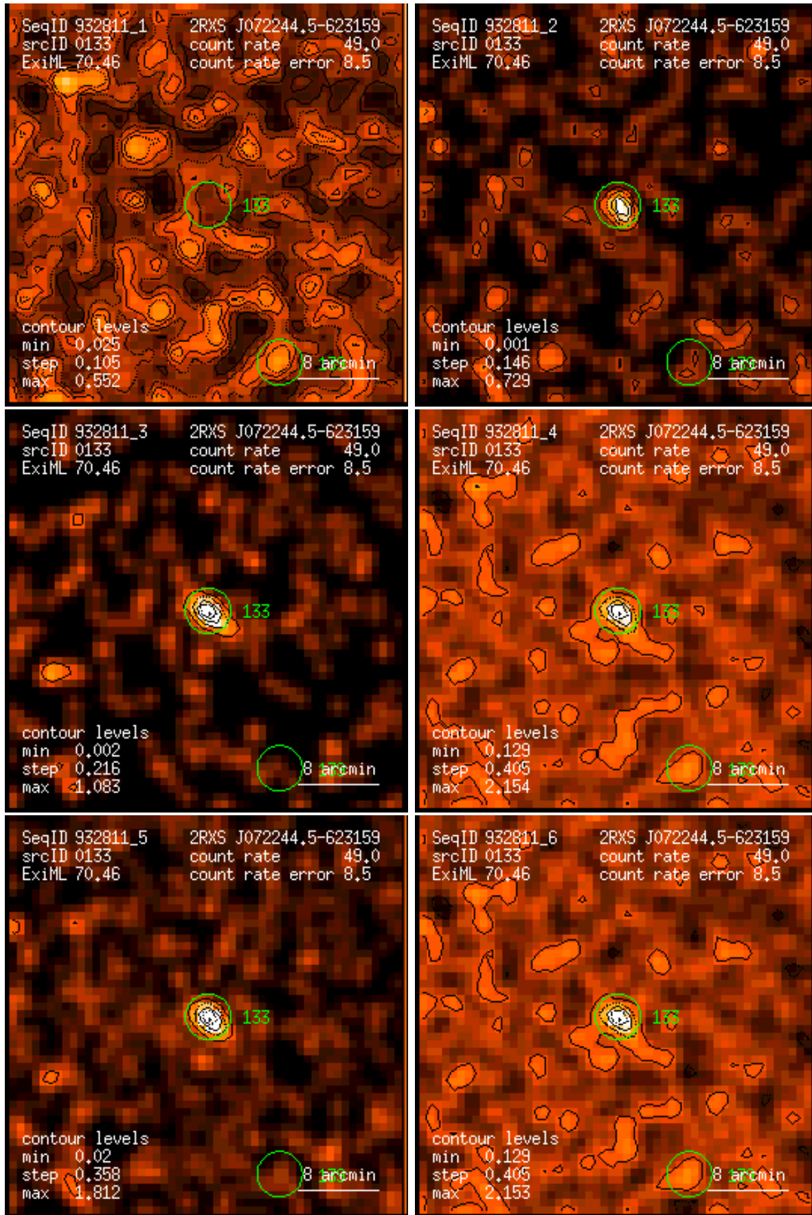
Figure 133: RASS 932811: detection 0133: band rate images, Gaussian filter: (1) PSPC channels 11 – 41, (2) 52 – 90, (3) 91 – 201, (4) 11 – 235, (5) 52 – 201, (6) 11 – 201. Broad band rates in counts/ks. Band rate contour levels in counts/ks/arcmin 2 .
