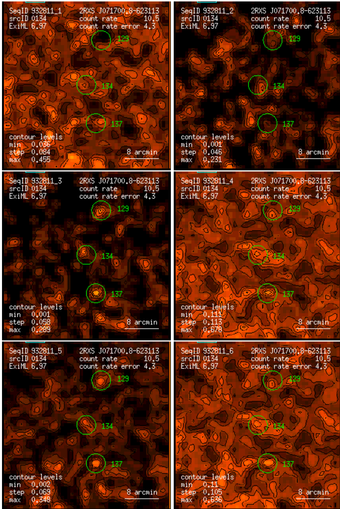
Figure 134: RASS 932811: detection 0134: band rate images, Gaussian filter: (1) PSPC channels 11 – 41, (2) 52 – 90, (3) 91 – 201, (4) 11 – 235, (5) 52 – 201, (6) 11 – 201. Broad band rates in counts/ks. Band rate contour levels in counts/ks/arcmin 2 .
