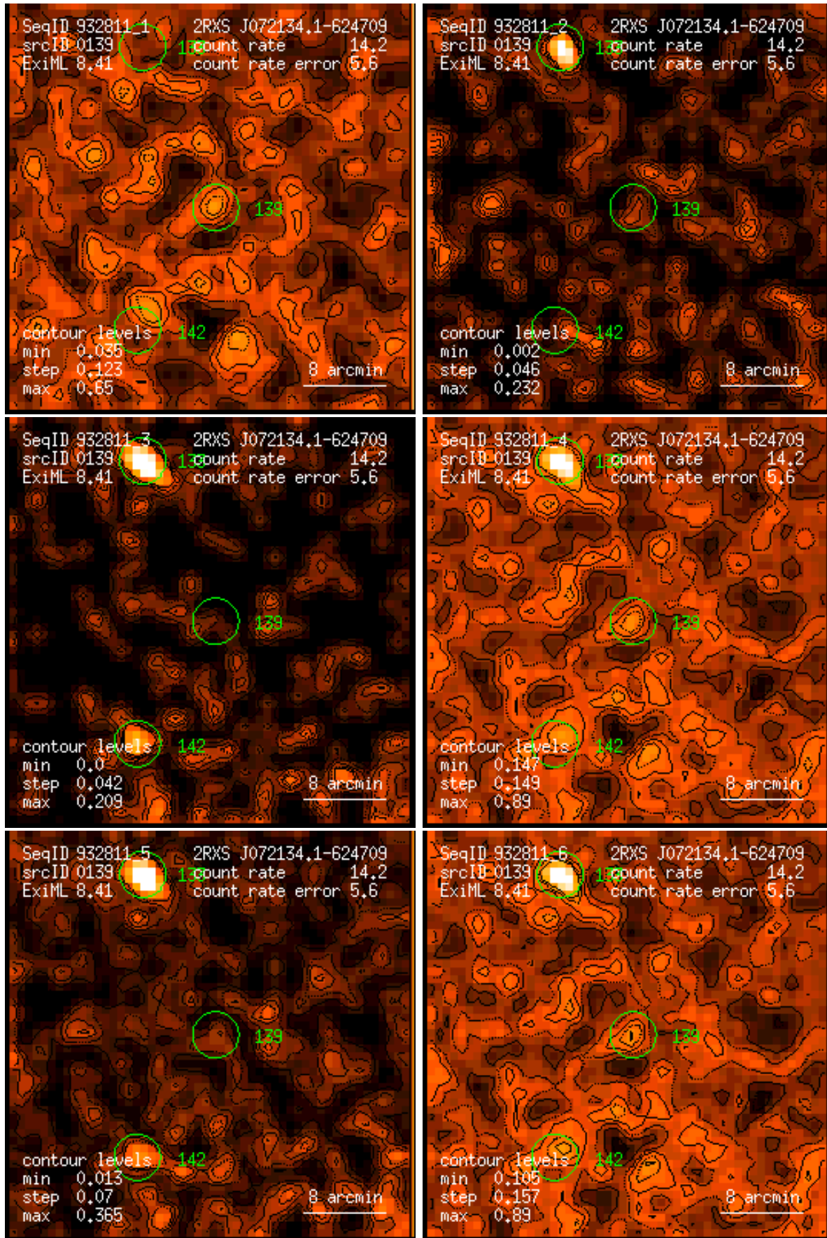
Figure 139: RASS 932811: detection 0139: band rate images, Gaussian filter: (1) PSPC channels 11 – 41, (2) 52 – 90, (3) 91 – 201, (4) 11 – 235, (5) 52 – 201, (6) 11 – 201. Broad band rates in counts/ks. Band rate contour levels in counts/ks/arcmin 2 .
