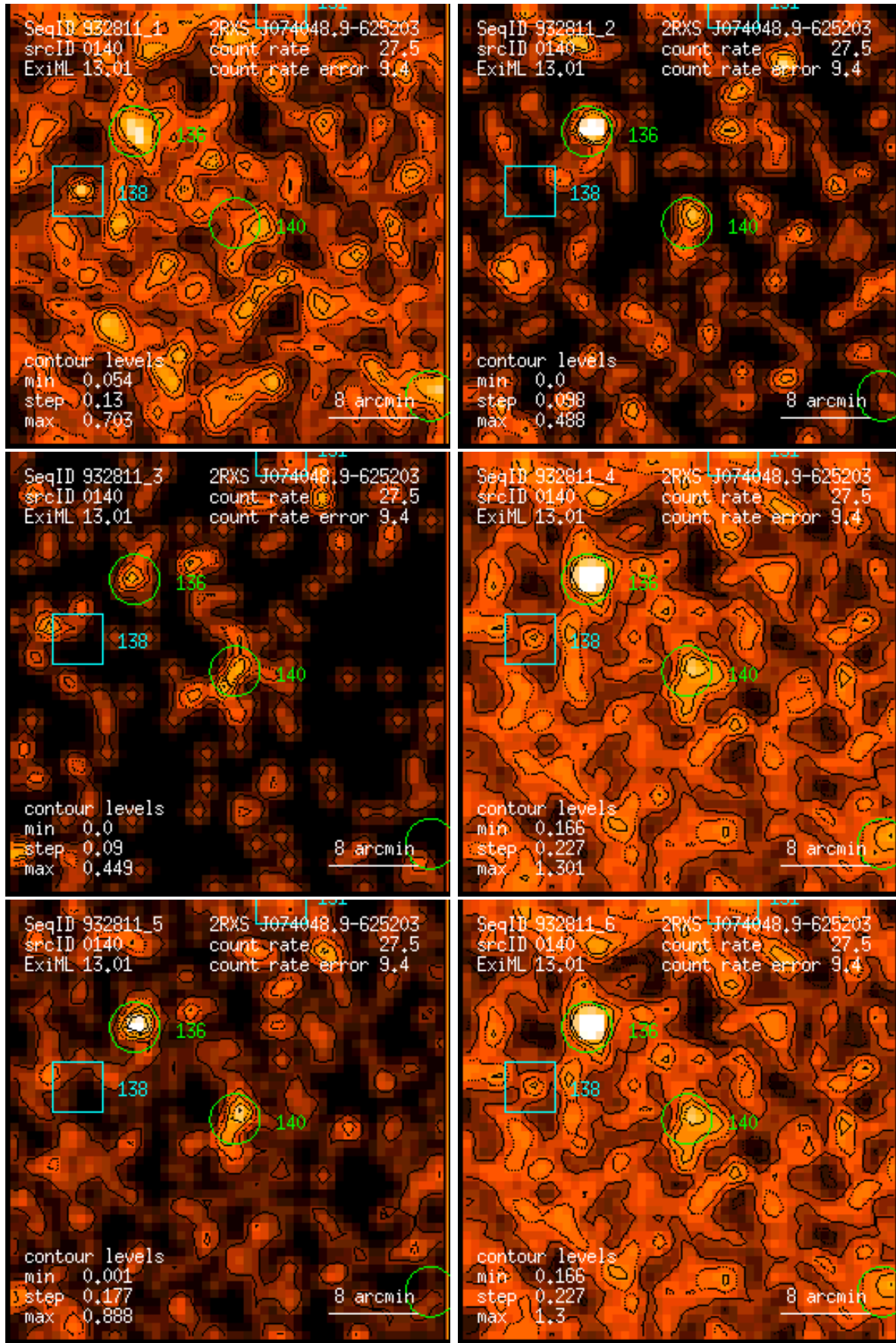
Figure 140: RASS 932811: detection 0140: band rate images, Gaussian filter: (1) PSPC channels 11 – 41, (2) 52 – 90, (3) 91 – 201, (4) 11 – 235, (5) 52 – 201, (6) 11 – 201. Broad band rates in counts/ks. Band rate contour levels in counts/ks/arcmin 2 .
