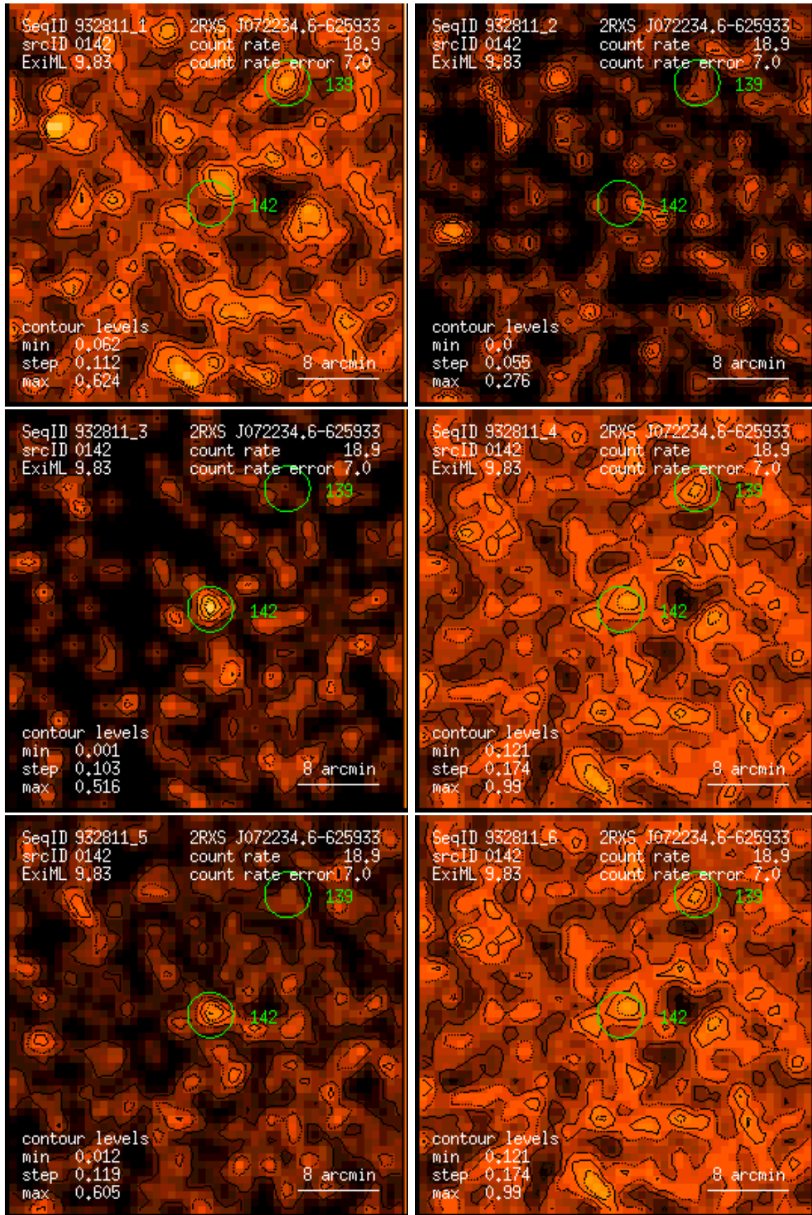
Figure 142: RASS 932811: detection 0142: band rate images, Gaussian filter: (1) PSPC channels 11 – 41, (2) 52 – 90, (3) 91 – 201, (4) 11 – 235, (5) 52 – 201, (6) 11 – 201. Broad band rates in counts/ks. Band rate contour levels in counts/ks/arcmin 2 .
