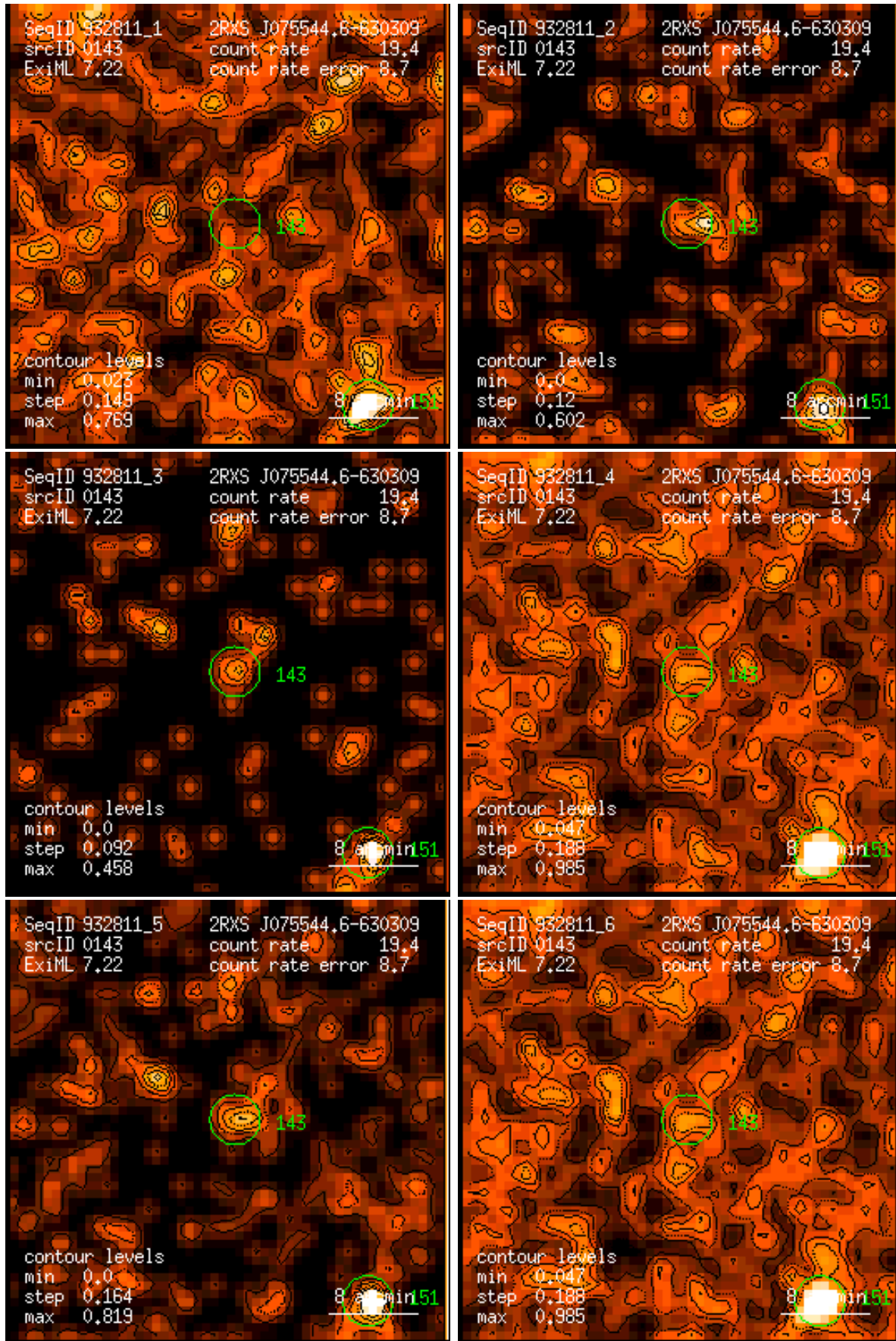
Figure 143: RASS 932811: detection 0143: band rate images, Gaussian filter: (1) PSPC channels 11 – 41, (2) 52 – 90, (3) 91 – 201, (4) 11 – 235, (5) 52 – 201, (6) 11 – 201. Broad band rates in counts/ks. Band rate contour levels in counts/ks/arcmin 2 .
