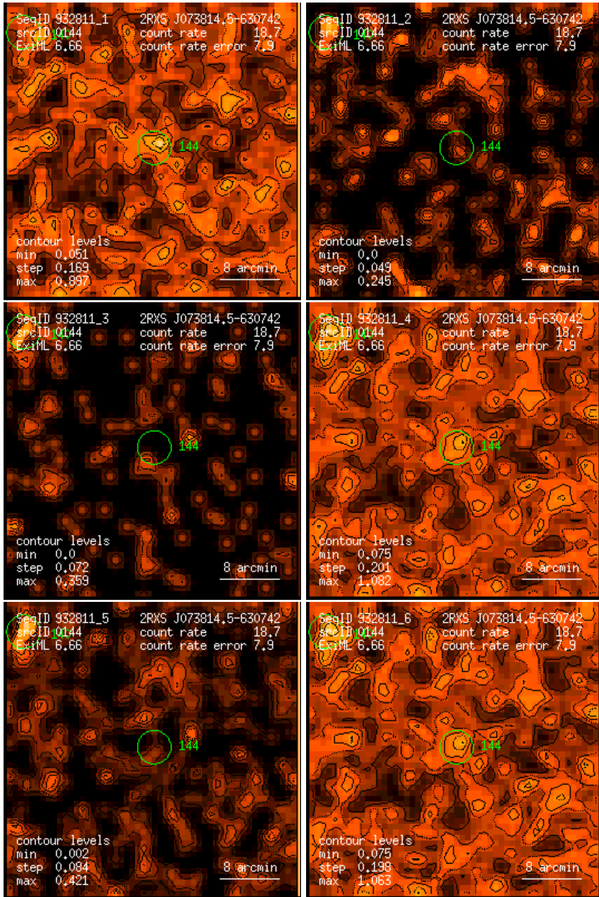
Figure 144: RASS 932811: detection 0144: band rate images, Gaussian filter: (1) PSPC channels 11 – 41, (2) 52 – 90, (3) 91 – 201, (4) 11 – 235, (5) 52 – 201, (6) 11 – 201. Broad band rates in counts/ks. Band rate contour levels in counts/ks/arcmin 2 .
