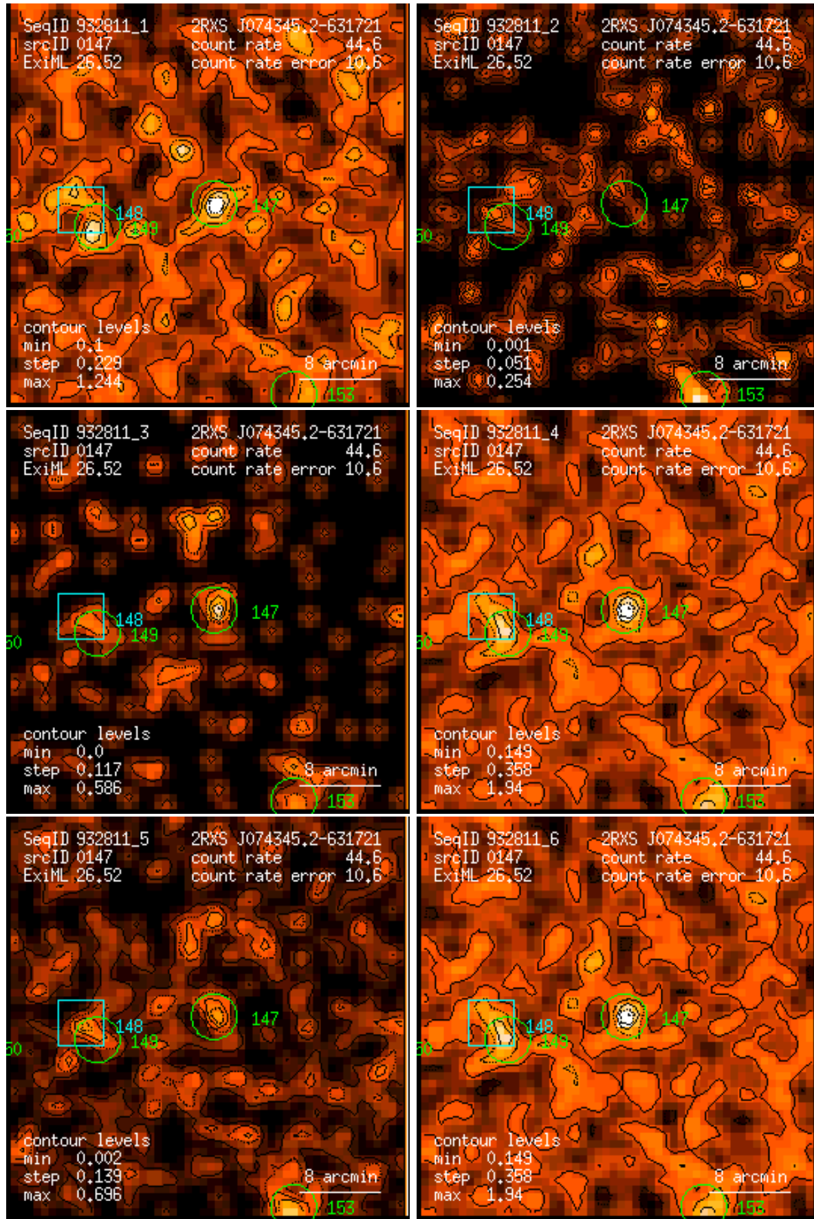
Figure 147: RASS 932811: detection 0147: band rate images, Gaussian filter: (1) PSPC channels 11 – 41, (2) 52 – 90, (3) 91 – 201, (4) 11 – 235, (5) 52 – 201, (6) 11 – 201. Broad band rates in counts/ks. Band rate contour levels in counts/ks/arcmin 2 .
