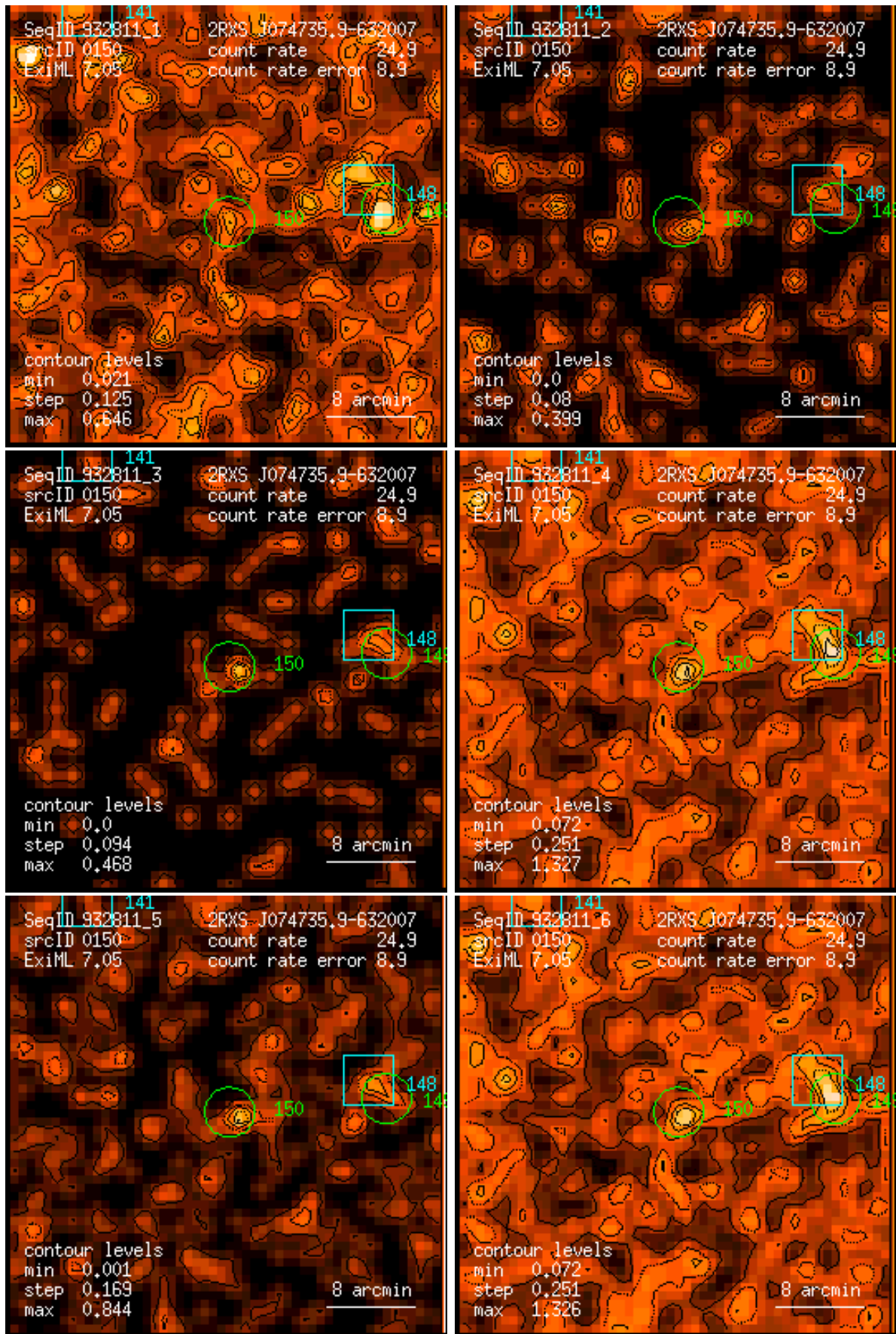
Figure 150: RASS 932811: detection 0150: band rate images, Gaussian filter: (1) PSPC channels 11 – 41, (2) 52 – 90, (3) 91 – 201, (4) 11 – 235, (5) 52 – 201, (6) 11 – 201. Broad band rates in counts/ks. Band rate contour levels in counts/ks/arcmin 2 .
