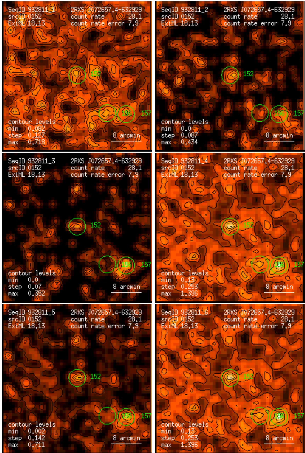
Figure 152: RASS 932811: detection 0152: band rate images, Gaussian filter: (1) PSPC channels 11 – 41, (2) 52 – 90, (3) 91 – 201, (4) 11 – 235, (5) 52 – 201, (6) 11 – 201. Broad band rates in counts/ks. Band rate contour levels in counts/ks/arcmin 2 .
