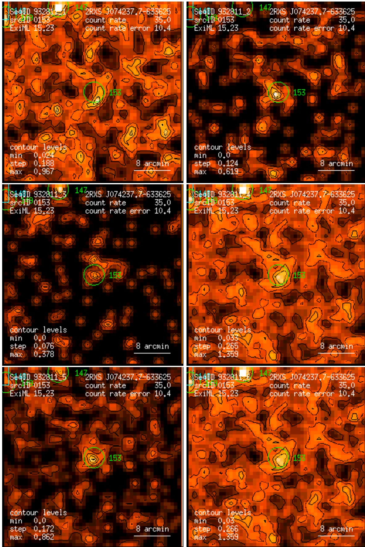
Figure 153: RASS 932811: detection 0153: band rate images, Gaussian filter: (1) PSPC channels 11 – 41, (2) 52 – 90, (3) 91 – 201, (4) 11 – 235, (5) 52 – 201, (6) 11 – 201. Broad band rates in counts/ks. Band rate contour levels in counts/ks/arcmin 2 .
