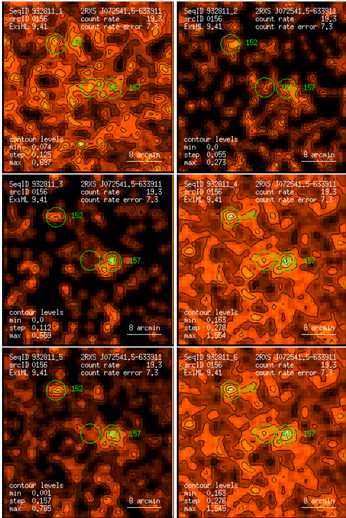
Figure 156: RASS 932811: detection 0156: band rate images, Gaussian filter: (1) PSPC channels 11 – 41, (2) 52 – 90, (3) 91 – 201, (4) 11 – 235, (5) 52 – 201, (6) 11 – 201. Broad band rates in counts/ks. Band rate contour levels in counts/ks/arcmin 2 .
