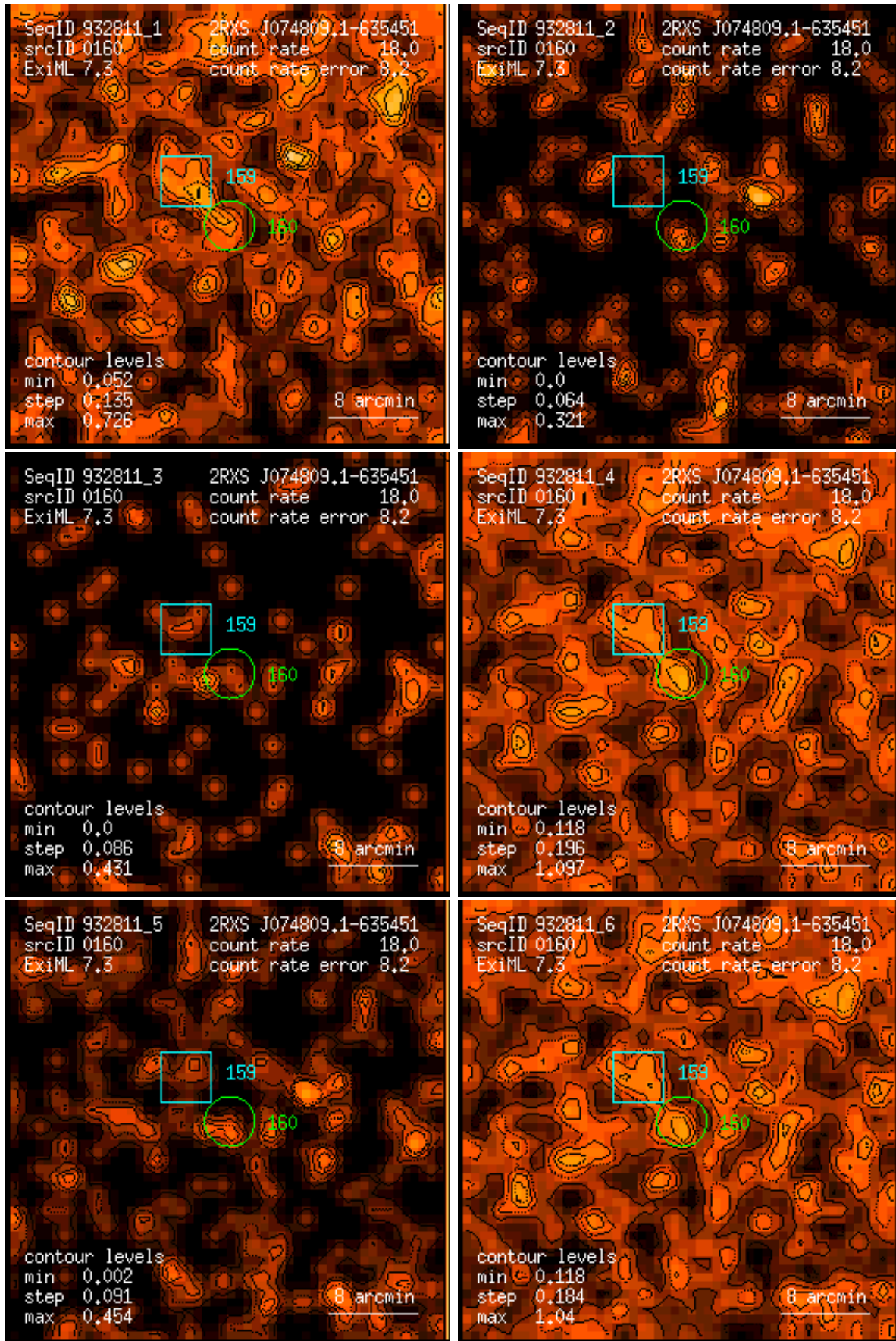
Figure 160: RASS 932811: detection 0160: band rate images, Gaussian filter: (1) PSPC channels 11 – 41, (2) 52 – 90, (3) 91 – 201, (4) 11 – 235, (5) 52 – 201, (6) 11 – 201. Broad band rates in counts/ks. Band rate contour levels in counts/ks/arcmin 2 .
