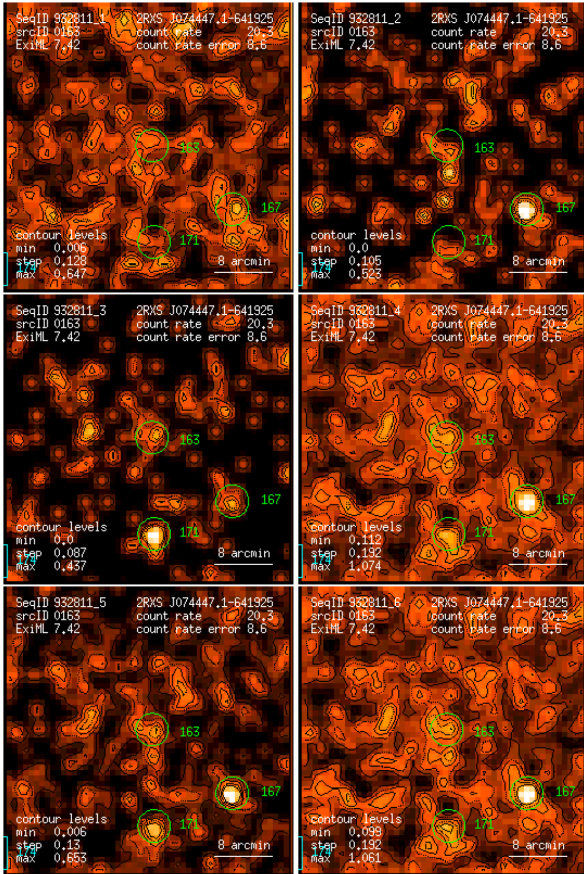
Figure 163: RASS 932811: detection 0163: band rate images, Gaussian filter: (1) PSPC channels 11 – 41, (2) 52 – 90, (3) 91 – 201, (4) 11 – 235, (5) 52 – 201, (6) 11 – 201. Broad band rates in counts/ks. Band rate contour levels in counts/ks/arcmin 2 .
