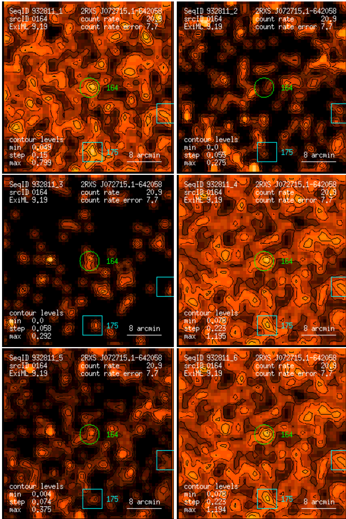
Figure 164: RASS 932811: detection 0164: band rate images, Gaussian filter: (1) PSPC channels 11 – 41, (2) 52 – 90, (3) 91 – 201, (4) 11 – 235, (5) 52 – 201, (6) 11 – 201. Broad band rates in counts/ks. Band rate contour levels in counts/ks/arcmin 2 .
