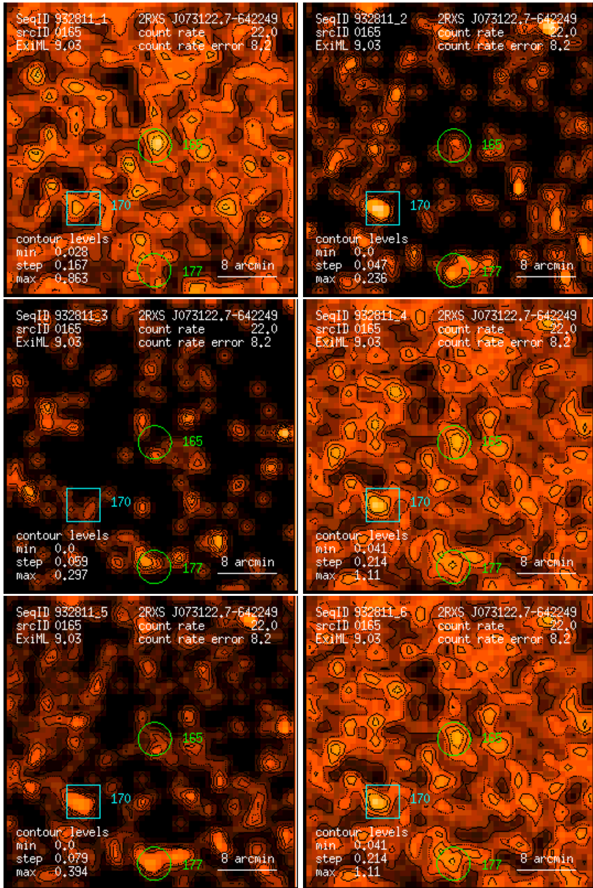
Figure 165: RASS 932811: detection 0165: band rate images, Gaussian filter: (1) PSPC channels 11 – 41, (2) 52 – 90, (3) 91 – 201, (4) 11 – 235, (5) 52 – 201, (6) 11 – 201. Broad band rates in counts/ks. Band rate contour levels in counts/ks/arcmin 2 .
