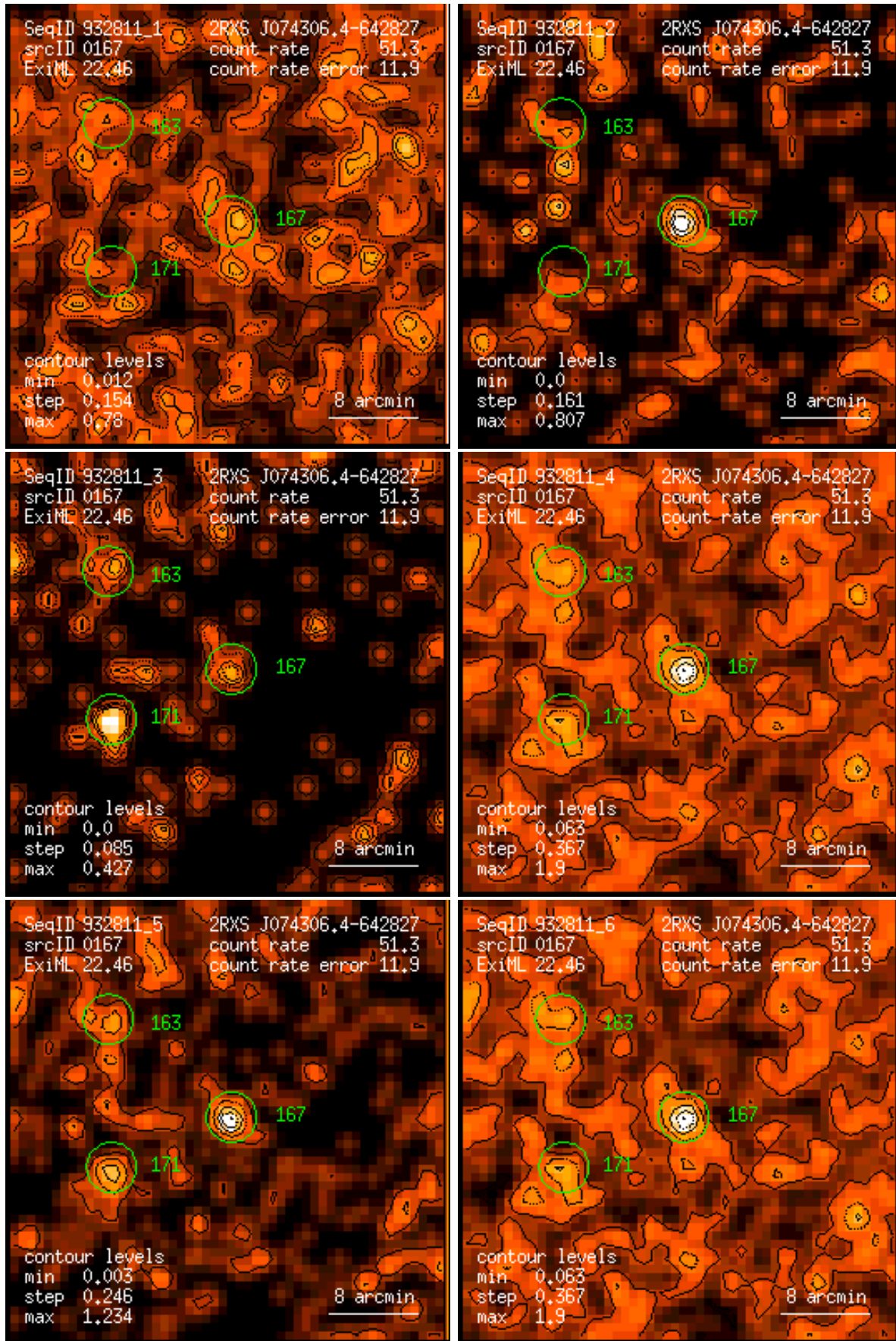
Figure 167: RASS 932811: detection 0167: band rate images, Gaussian filter: (1) PSPC channels 11 – 41, (2) 52 – 90, (3) 91 – 201, (4) 11 – 235, (5) 52 – 201, (6) 11 – 201. Broad band rates in counts/ks. Band rate contour levels in counts/ks/arcmin 2 .
