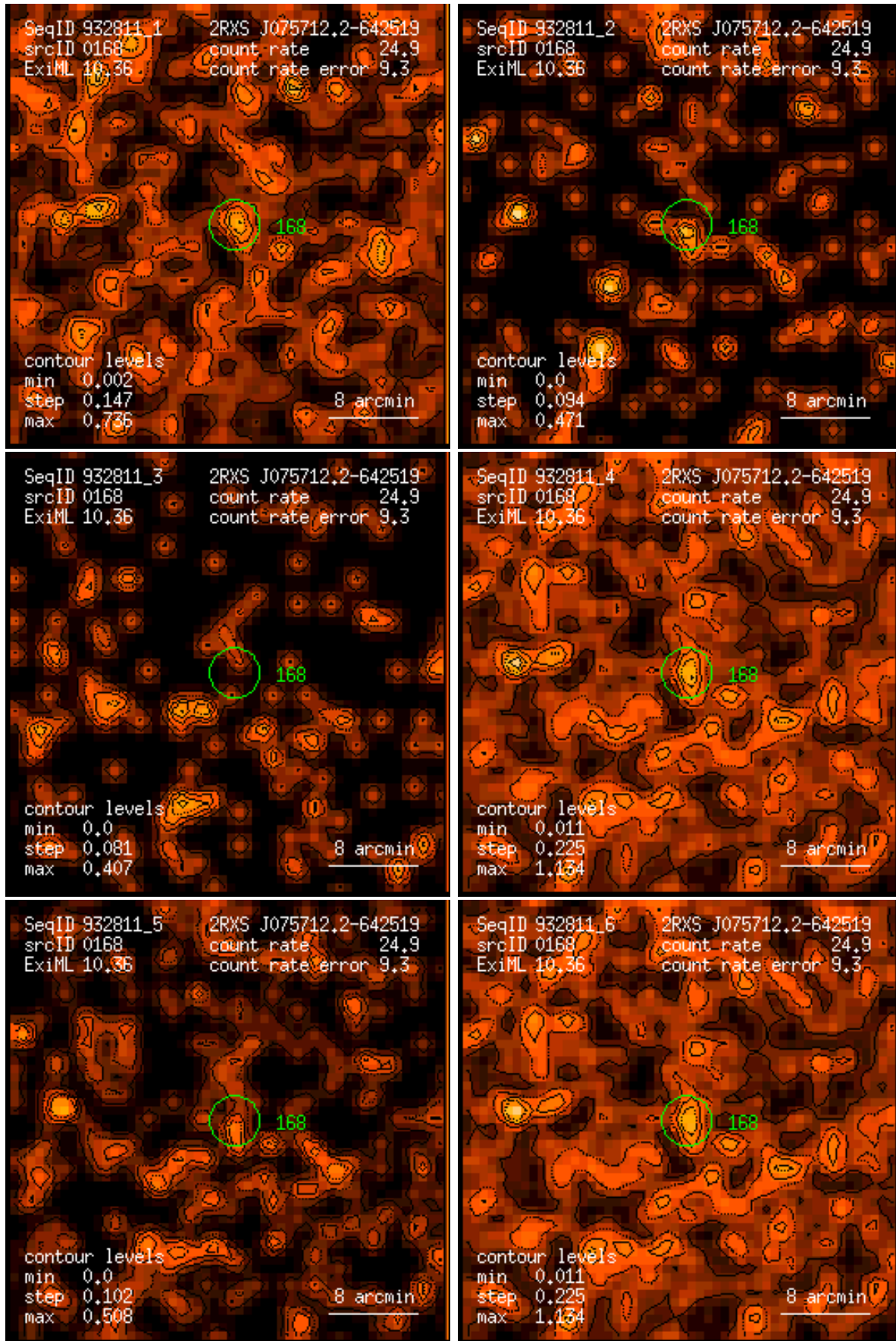
Figure 168: RASS 932811: detection 0168: band rate images, Gaussian filter: (1) PSPC channels 11 – 41, (2) 52 – 90, (3) 91 – 201, (4) 11 – 235, (5) 52 – 201, (6) 11 – 201. Broad band rates in counts/ks. Band rate contour levels in counts/ks/arcmin 2 .
