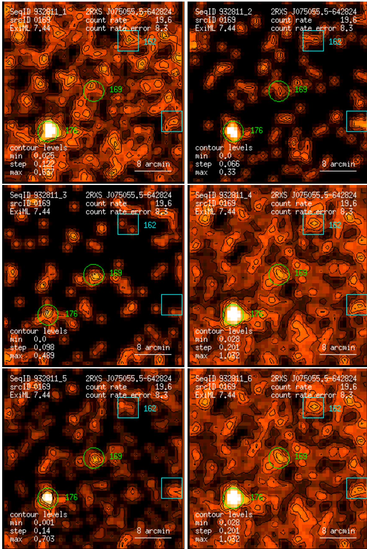
Figure 169: RASS 932811: detection 0169: band rate images, Gaussian filter: (1) PSPC channels 11 – 41, (2) 52 – 90, (3) 91 – 201, (4) 11 – 235, (5) 52 – 201, (6) 11 – 201. Broad band rates in counts/ks. Band rate contour levels in counts/ks/arcmin 2 .
