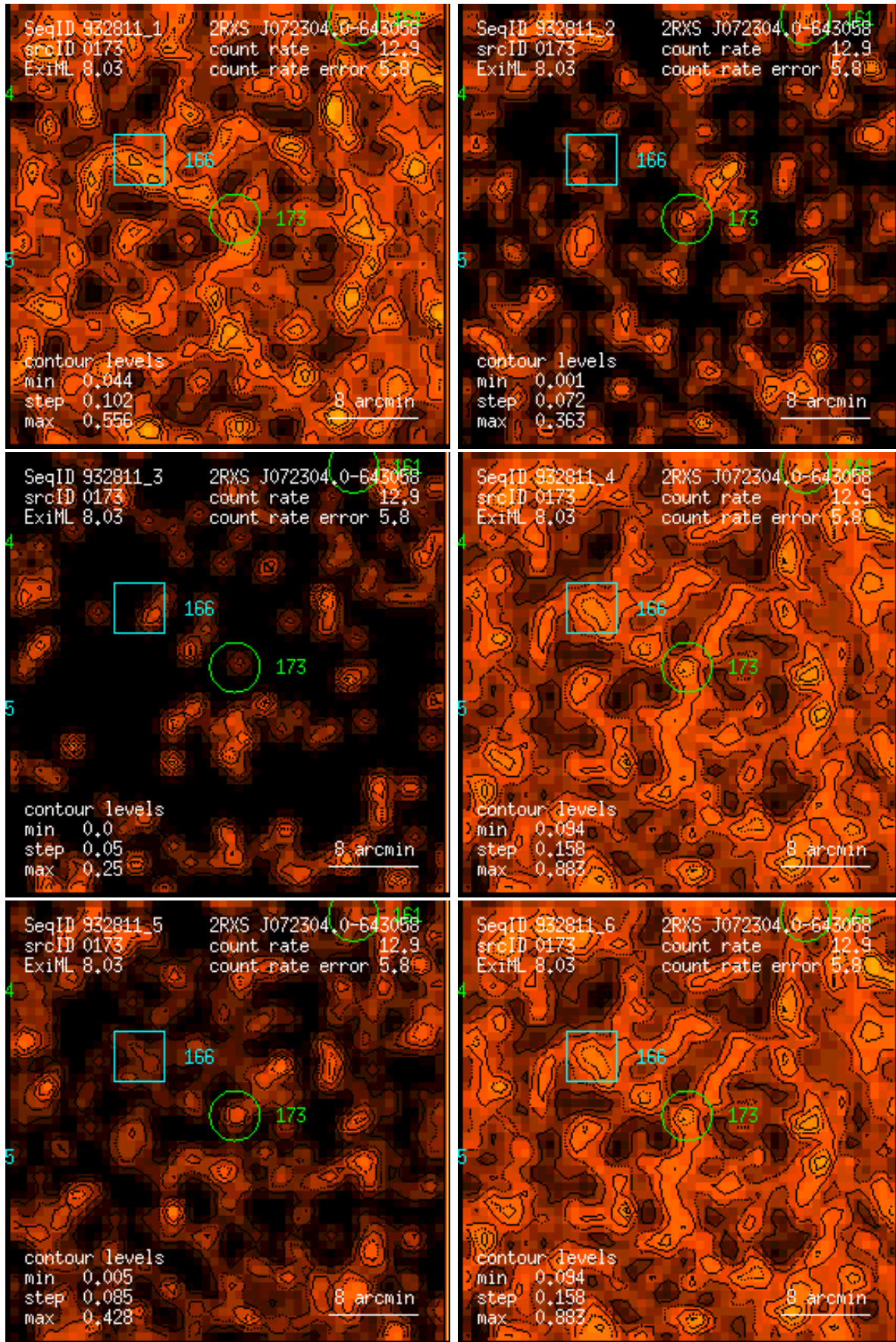
Figure 173: RASS 932811: detection 0173: band rate images, Gaussian filter: (1) PSPC channels 11 – 41, (2) 52 – 90, (3) 91 – 201, (4) 11 – 235, (5) 52 – 201, (6) 11 – 201. Broad band rates in counts/ks. Band rate contour levels in counts/ks/arcmin 2 .
