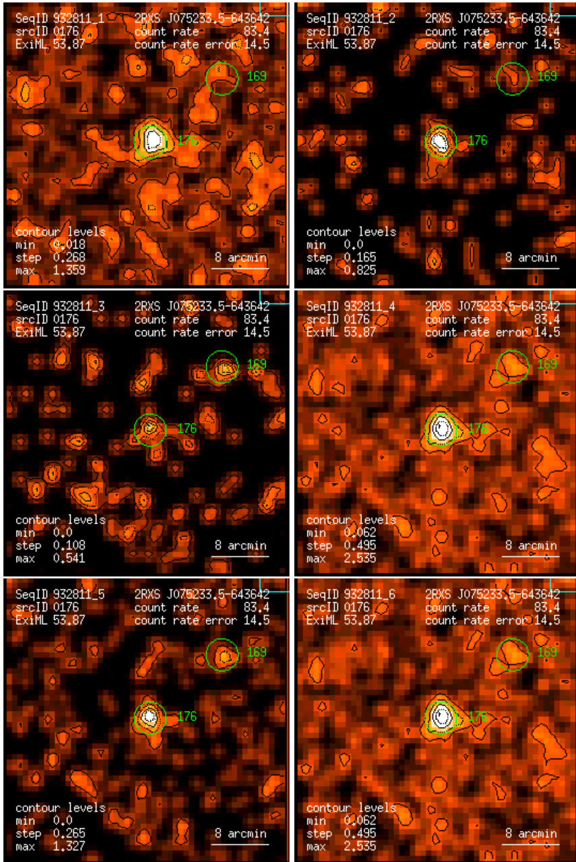
Figure 176: RASS 932811: detection 0176: band rate images, Gaussian filter: (1) PSPC channels 11 – 41, (2) 52 – 90, (3) 91 – 201, (4) 11 – 235, (5) 52 – 201, (6) 11 – 201. Broad band rates in counts/ks. Band rate contour levels in counts/ks/arcmin 2 .
