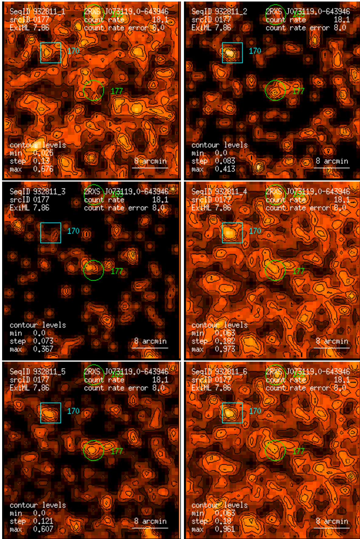
Figure 177: RASS 932811: detection 0177: band rate images, Gaussian filter: (1) PSPC channels 11 – 41, (2) 52 – 90, (3) 91 – 201, (4) 11 – 235, (5) 52 – 201, (6) 11 – 201. Broad band rates in counts/ks. Band rate contour levels in counts/ks/arcmin 2 .
