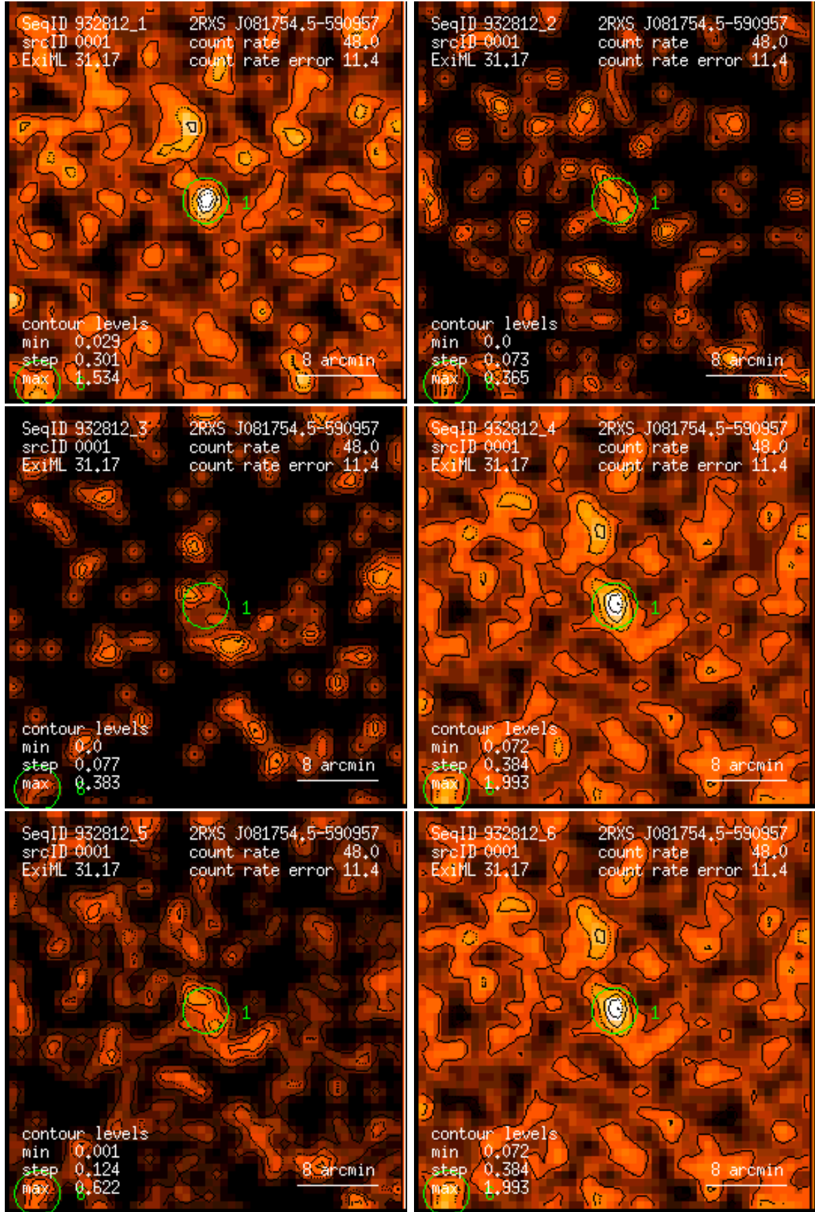
Figure 1: RASS 932812: detection 0001: band rate images, Gaussian filter: (1) PSPC channels 11 – 41, (2) 52 – 90, (3) 91 – 201, (4) 11 – 235, (5) 52 – 201, (6) 11 – 201. Broad band rates in counts/ks. Band rate contour levels in counts/ks/arcmin 2 .
