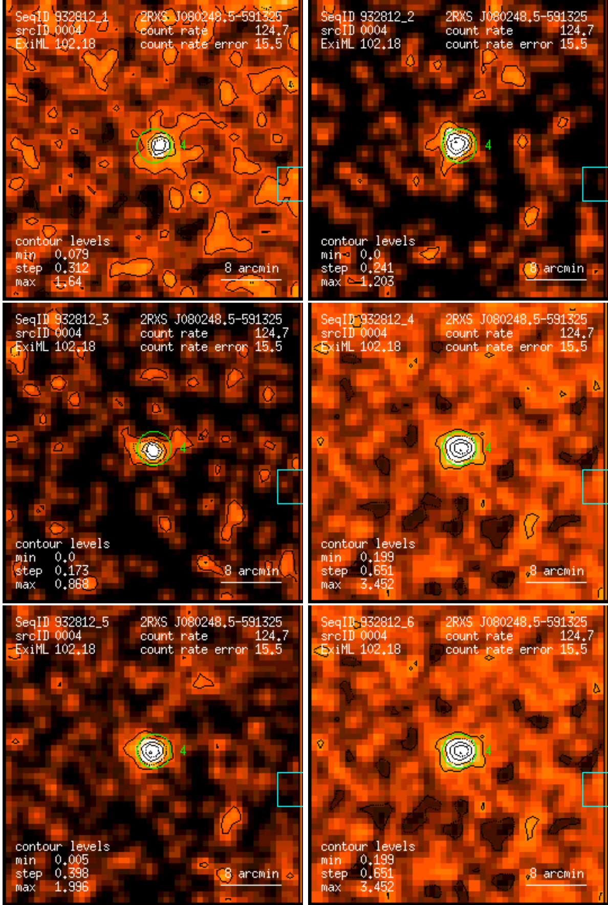
Figure 4: RASS 932812: detection 0004: band rate images, Gaussian filter: (1) PSPC channels 11 – 41, (2) 52 – 90, (3) 91 – 201, (4) 11 – 235, (5) 52 – 201, (6) 11 – 201. Broad band rates in counts/ks. Band rate contour levels in counts/ks/arcmin 2 .
