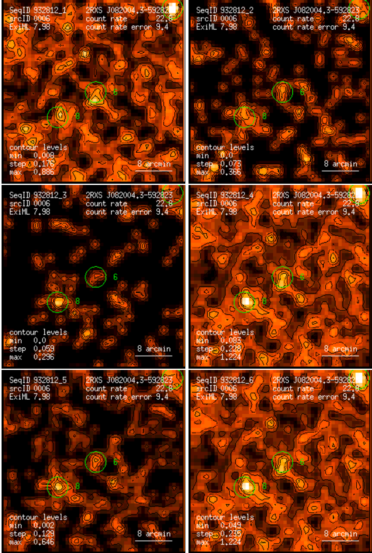
Figure 6: RASS 932812: detection 0006: band rate images, Gaussian filter: (1) PSPC channels 11 – 41, (2) 52 – 90, (3) 91 – 201, (4) 11 – 235, (5) 52 – 201, (6) 11 – 201. Broad band rates in counts/ks. Band rate contour levels in counts/ks/arcmin 2 .
