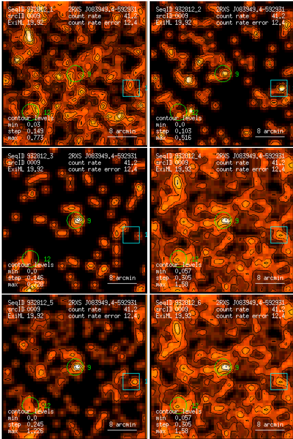
Figure 9: RASS 932812: detection 0009: band rate images, Gaussian filter: (1) PSPC channels 11 – 41, (2) 52 – 90, (3) 91 – 201, (4) 11 – 235, (5) 52 – 201, (6) 11 – 201. Broad band rates in counts/ks. Band rate contour levels in counts/ks/arcmin 2 .
