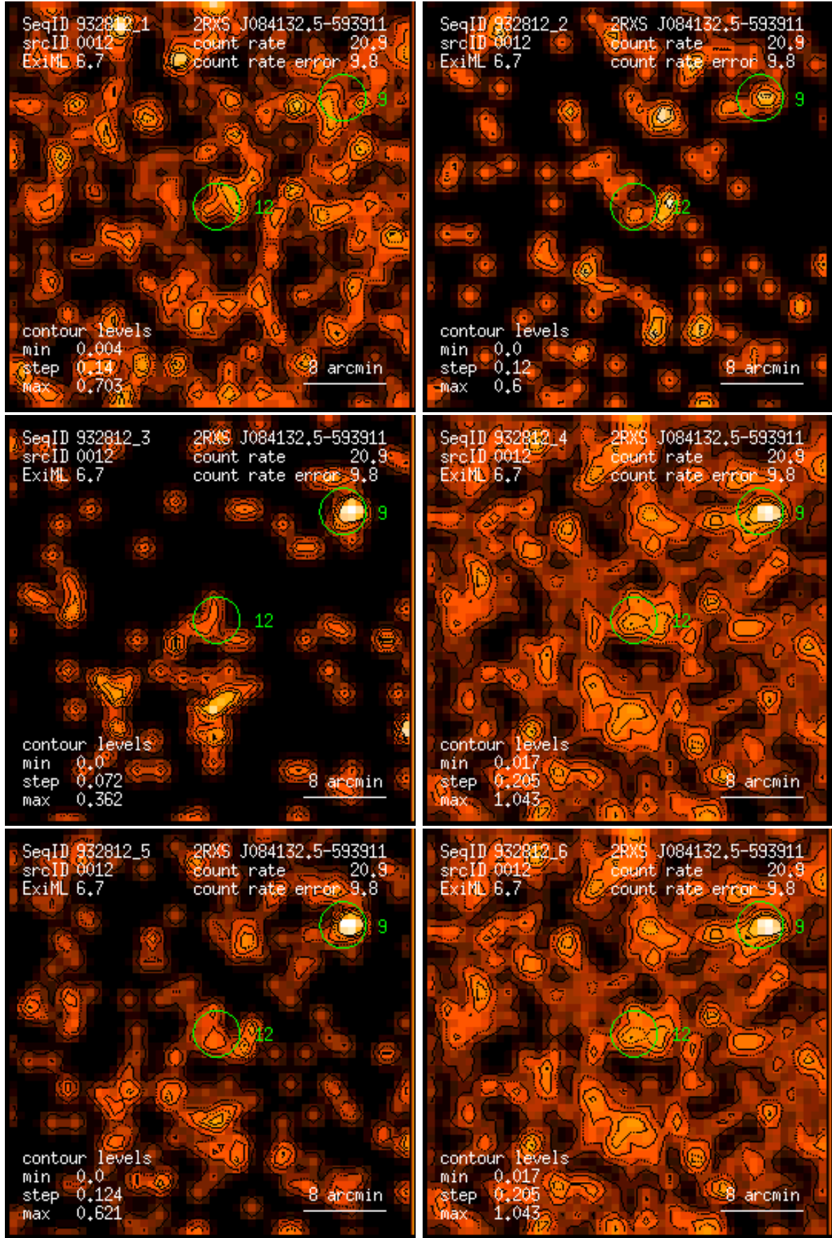
Figure 12: RASS 932812: detection 0012: band rate images, Gaussian filter: (1) PSPC channels 11 – 41, (2) 52 – 90, (3) 91 – 201, (4) 11 – 235, (5) 52 – 201, (6) 11 – 201. Broad band rates in counts/ks. Band rate contour levels in counts/ks/arcmin 2 .
