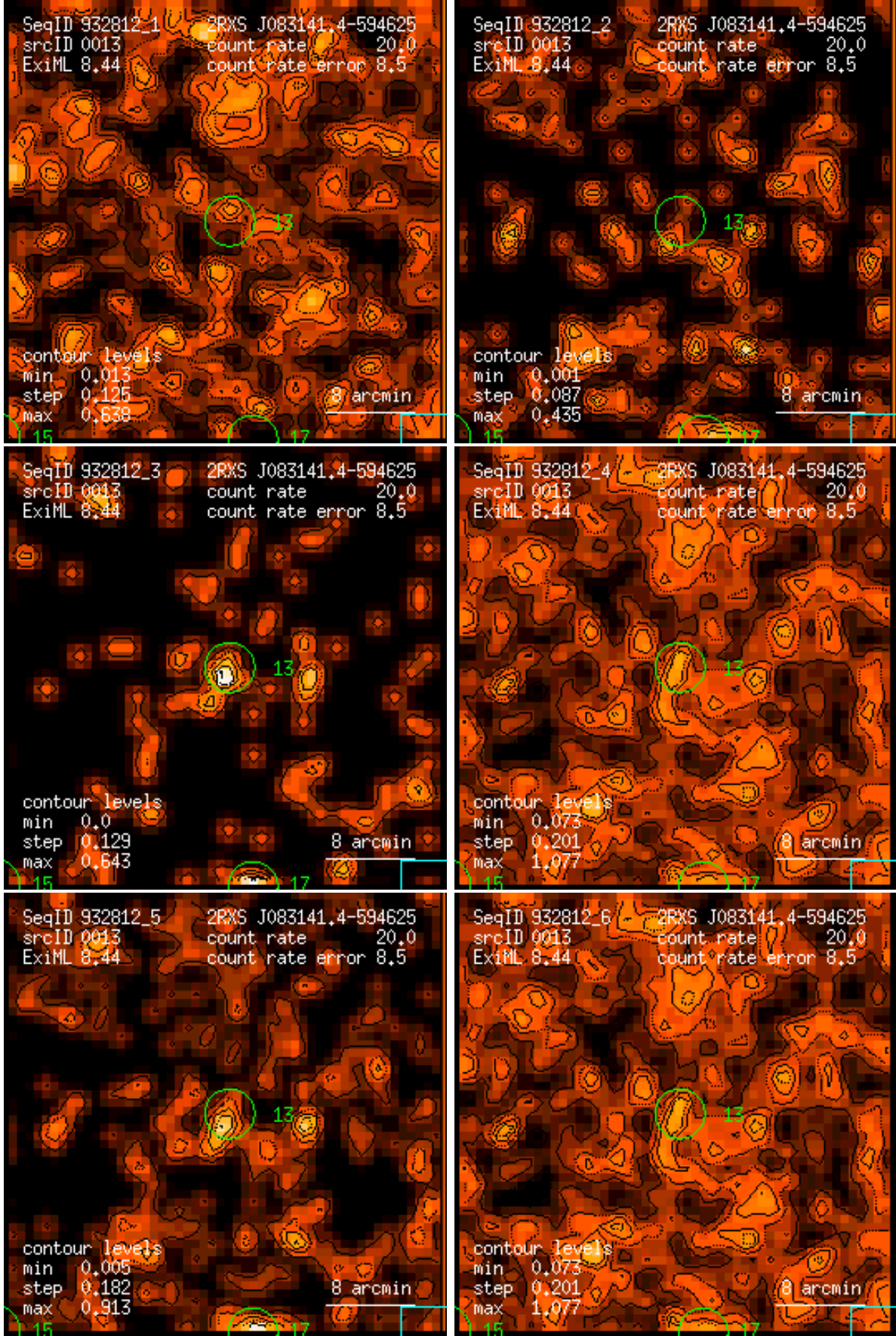
Figure 13: RASS 932812: detection 0013: band rate images, Gaussian filter: (1) PSPC channels 11 – 41, (2) 52 – 90, (3) 91 – 201, (4) 11 – 235, (5) 52 – 201, (6) 11 – 201. Broad band rates in counts/ks. Band rate contour levels in counts/ks/arcmin 2 .
