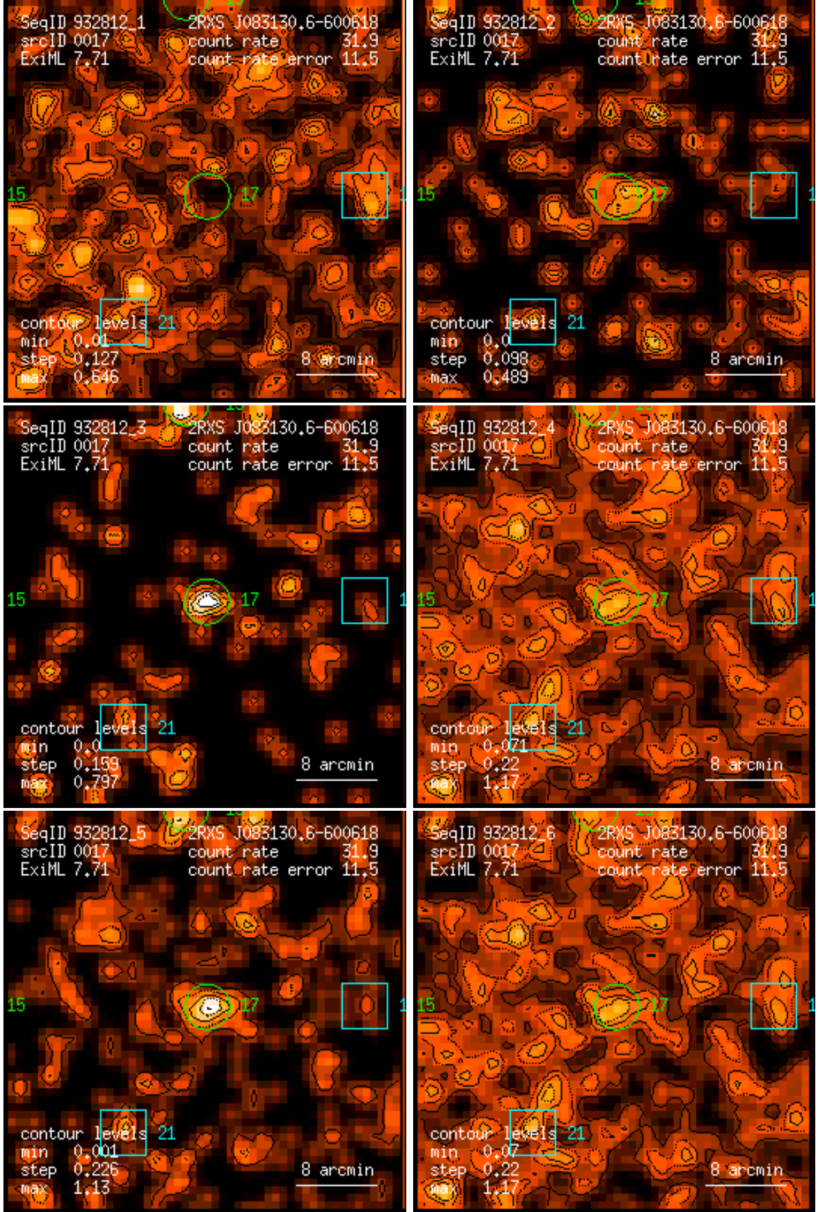
Figure 17: RASS 932812: detection 0017: band rate images, Gaussian filter: (1) PSPC channels 11 – 41, (2) 52 – 90, (3) 91 – 201, (4) 11 – 235, (5) 52 – 201, (6) 11 – 201. Broad band rates in counts/ks. Band rate contour levels in counts/ks/arcmin 2 .
