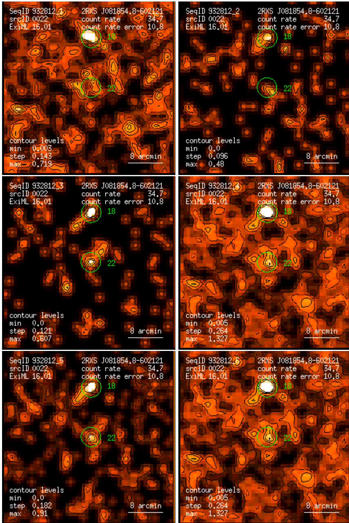
Figure 22: RASS 932812: detection 0022: band rate images, Gaussian filter: (1) PSPC channels 11 – 41, (2) 52 – 90, (3) 91 – 201, (4) 11 – 235, (5) 52 – 201, (6) 11 – 201. Broad band rates in counts/ks. Band rate contour levels in counts/ks/arcmin 2 .
