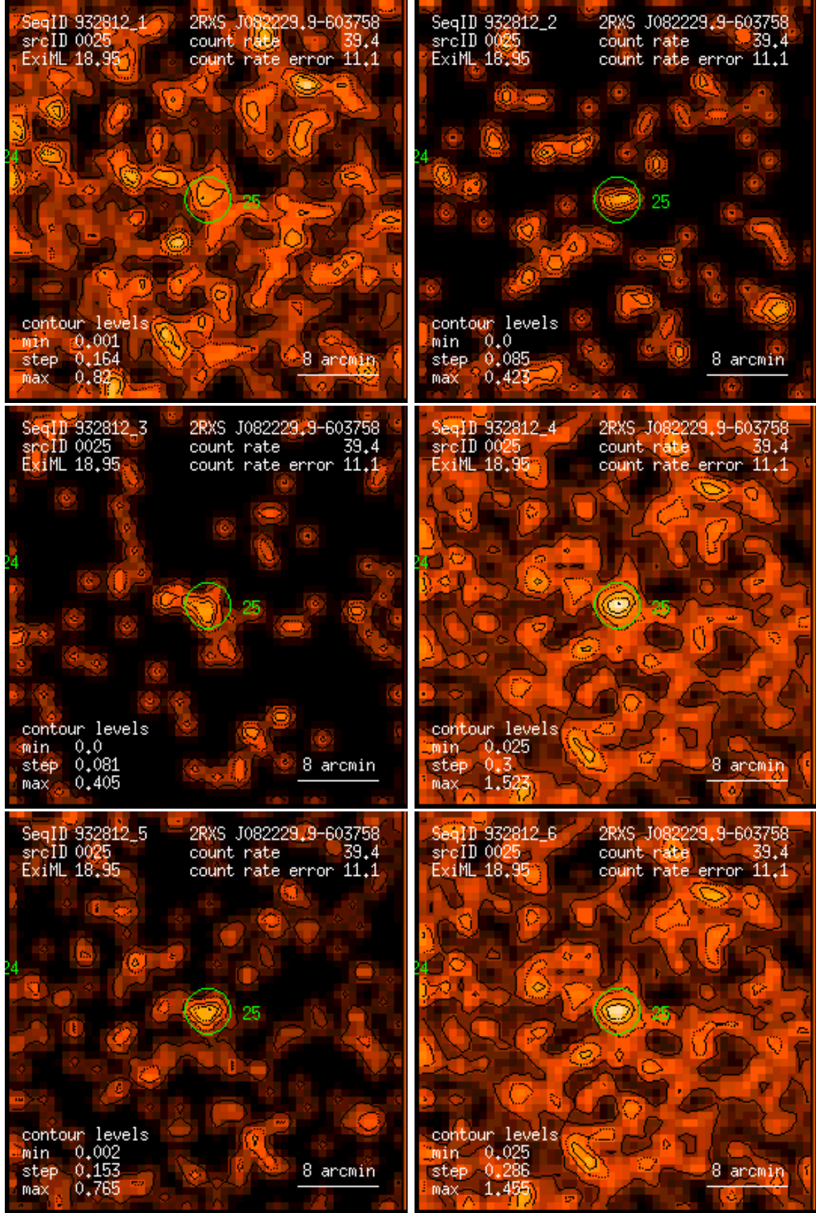
Figure 25: RASS 932812: detection 0025: band rate images, Gaussian filter: (1) PSPC channels 11 – 41, (2) 52 – 90, (3) 91 – 201, (4) 11 – 235, (5) 52 – 201, (6) 11 – 201. Broad band rates in counts/ks. Band rate contour levels in counts/ks/arcmin 2 .
